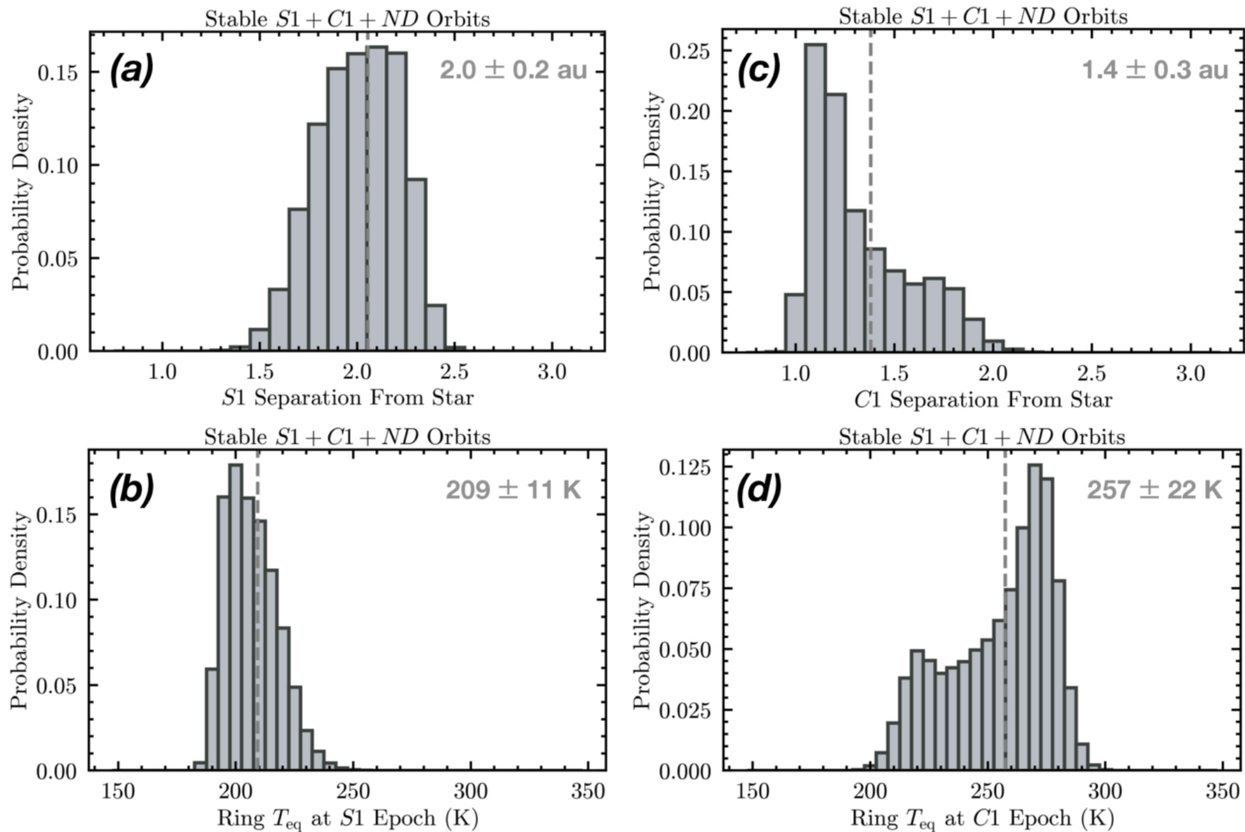
Figure 14. from Charles Beichman et al 2025 Astrophys. J. Lett. 989 doi:10.3847/2041-8213/adf53f https://dx.doi.org/10.3847/2041-8213/adf53f © 2025. The Author(s). Published by the American Astronomical Society.
