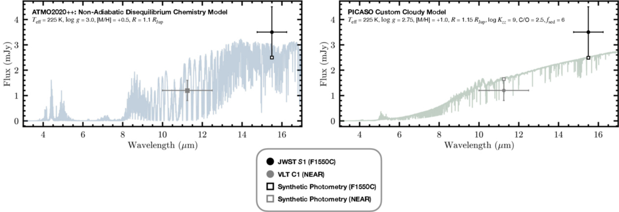
Figure 13. from Charles Beichman et al 2025 Astrophys. J. Lett. 989 doi:10.3847/2041-8213/adf53f https://dx.doi.org/10.3847/2041-8213/adf53f © 2025. The Author(s). Published by the American Astronomical Society.
