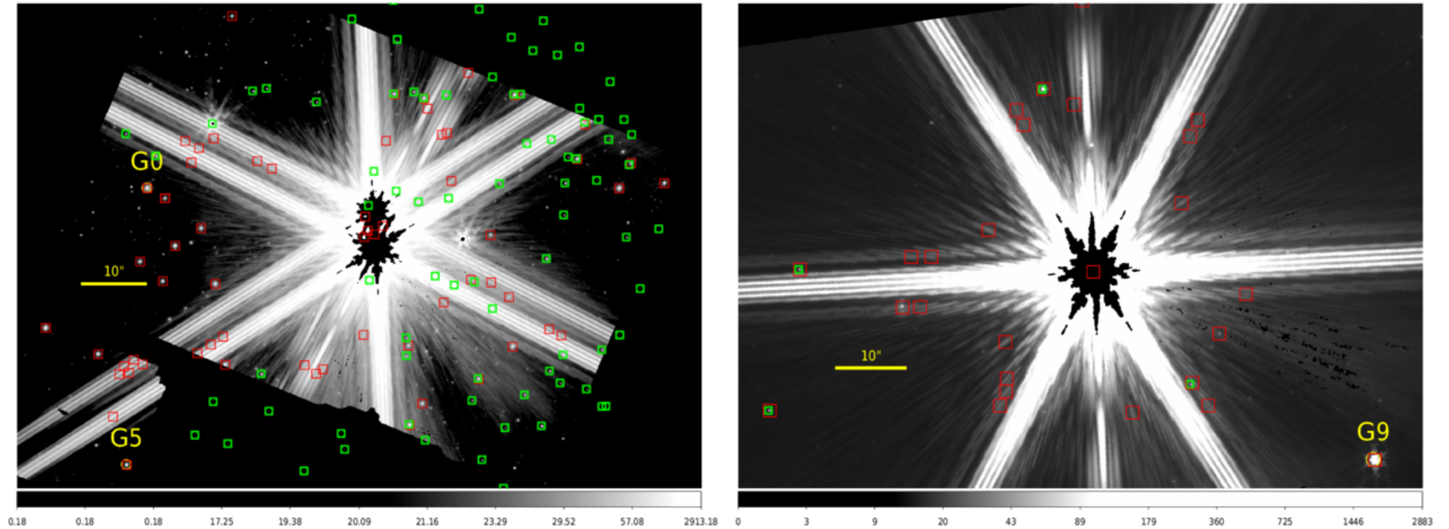
Figure 1. from Charles Beichman et al 2025 Astrophys. J. Lett. 989 doi:10.3847/2041-8213/adf53f https://dx.doi.org/10.3847/2041-8213/adf53f © 2025. The Author(s). Published by the American Astronomical Society.
