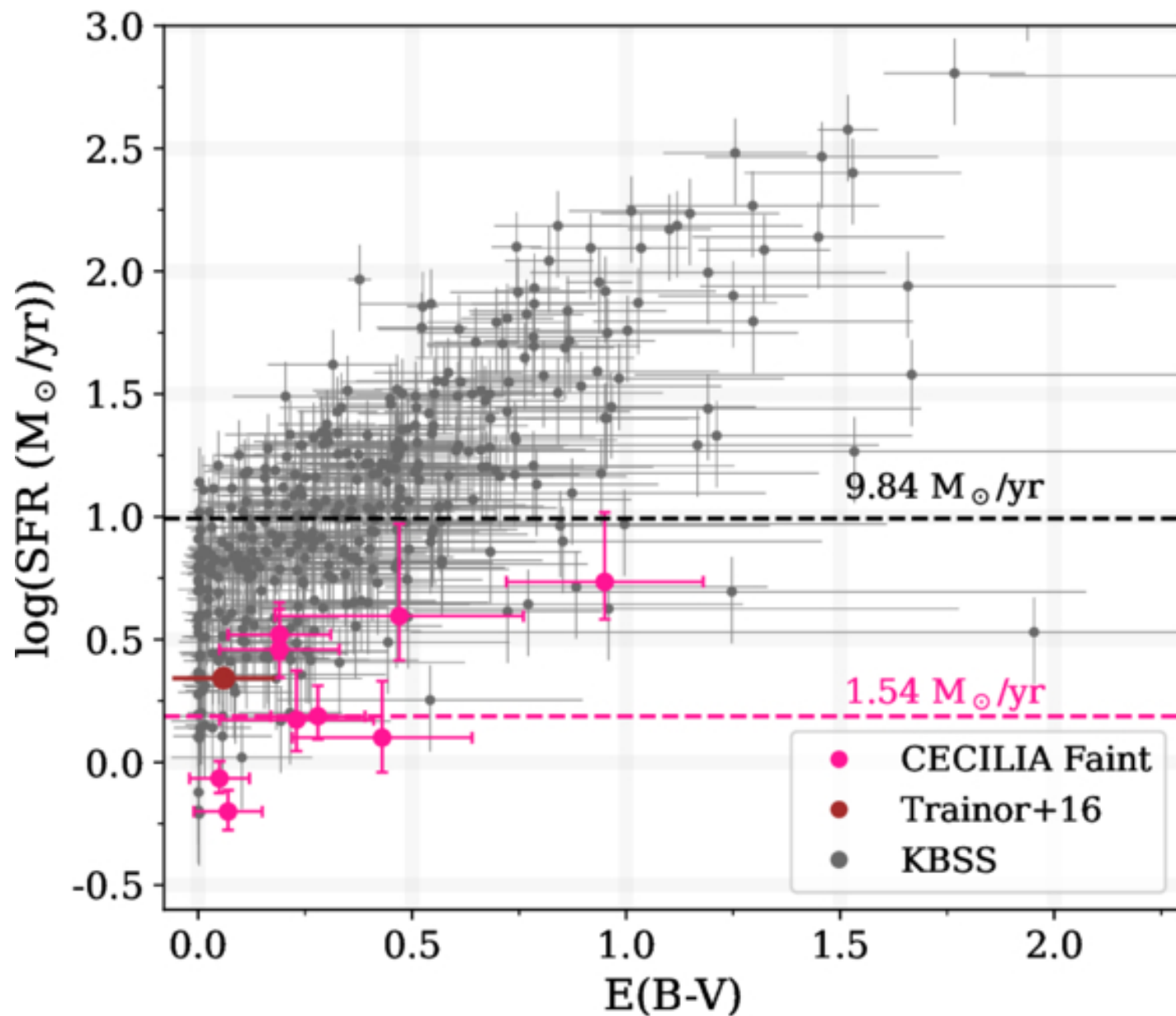
Figure 5. from Menelaos Raptis et al 2025 Astrophys. J. Lett. 989 doi:10.3847/2041-8213/adf4eb https://dx.doi.org/10.3847/2041-8213/adf4eb © 2025. The Author(s). Published by the American Astronomical Society.
