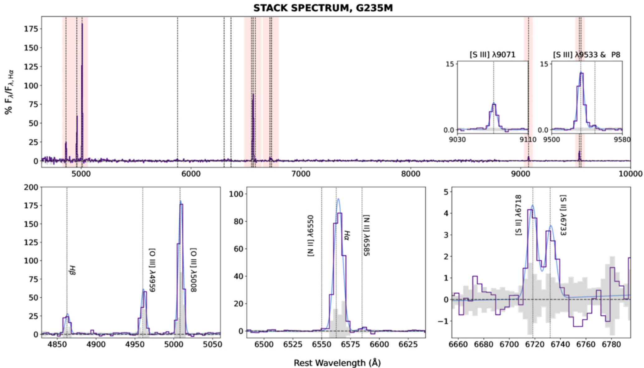
Figure 3. from Menelaos Raptis et al 2025 Astrophys. J. Lett. 989 doi:10.3847/2041-8213/adf4eb https://dx.doi.org/10.3847/2041-8213/adf4eb © 2025. The Author(s). Published by the American Astronomical Society.
