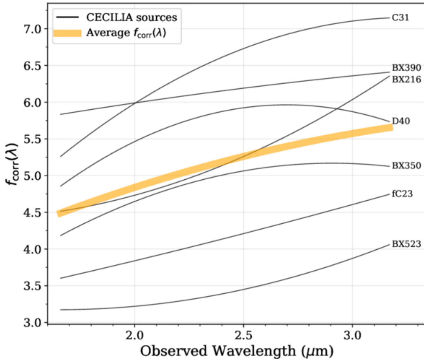
Figure 2. from Menelaos Raptis et al 2025 Astrophys. J. Lett. 989 doi:10.3847/2041-8213/adf4eb https://dx.doi.org/10.3847/2041-8213/adf4eb © 2025. The Author(s). Published by the American Astronomical Society.
