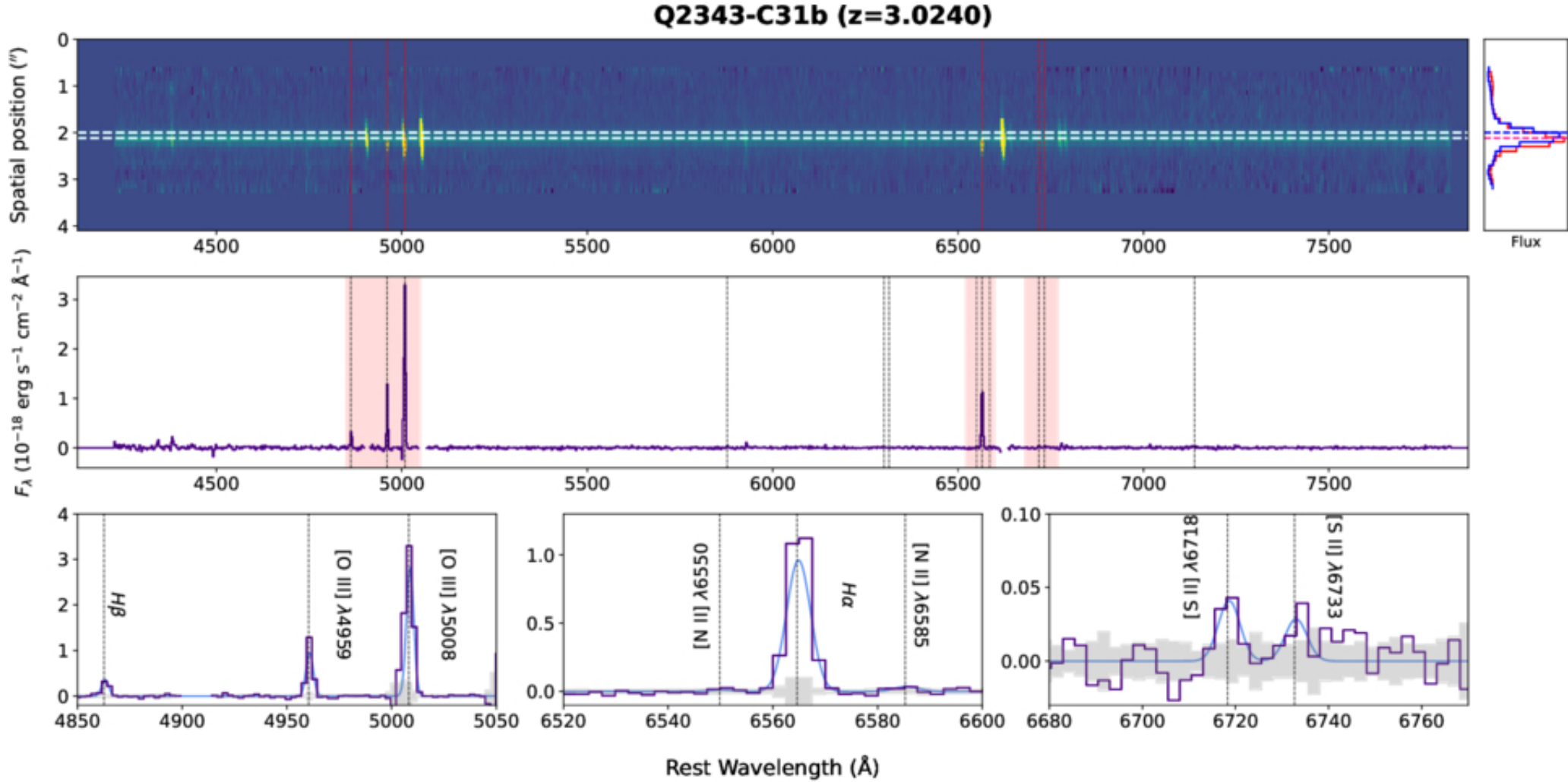
Figure 12. from Menelaos Raptis et al 2025 Astrophys. J. Lett. 989 doi:10.3847/2041-8213/adf4eb https://dx.doi.org/10.3847/2041-8213/adf4eb © 2025. The Author(s). Published by the American Astronomical Society.
