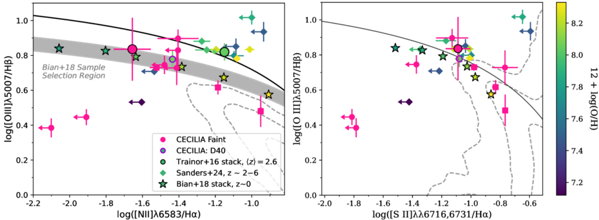
Figure 10. from Menelaos Raptis et al 2025 Astrophys. J. Lett. 989 doi:10.3847/2041-8213/adf4eb https://dx.doi.org/10.3847/2041-8213/adf4eb © 2025. The Author(s). Published by the American Astronomical Society.
