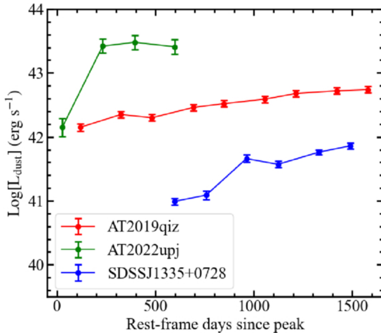
Figure 6. from Mingxin Wu et al 2025 Astrophys. J. Lett. 988 doi:10.3847/2041-8213/adf229 https://dx.doi.org/10.3847/2041-8213/adf229 © 2025. The Author(s). Published by the American Astronomical Society.
