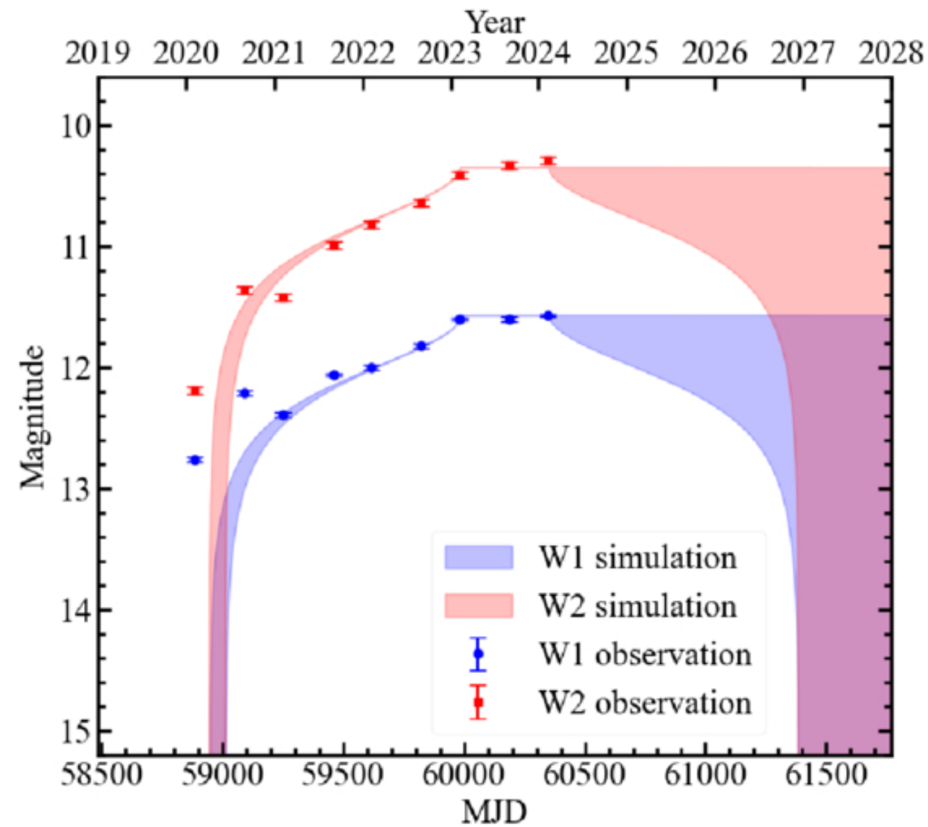
Figure 5. from Mingxin Wu et al 2025 Astrophys. J. Lett. 988 doi:10.3847/2041-8213/adf229 https://dx.doi.org/10.3847/2041-8213/adf229 © 2025. The Author(s). Published by the American Astronomical Society.
