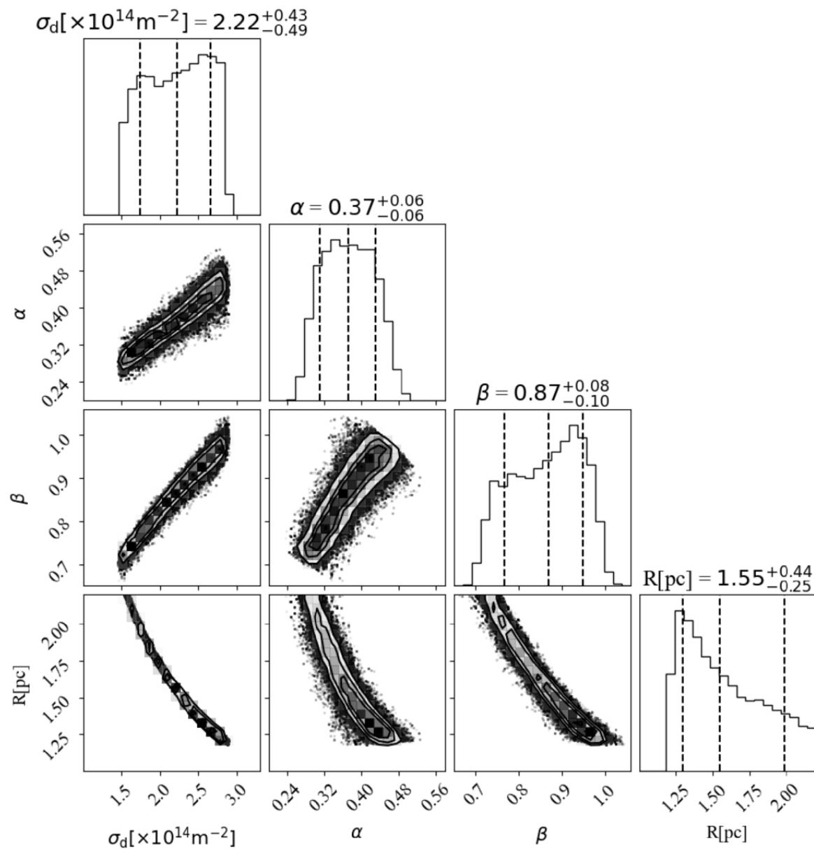
Figure 4. from Mingxin Wu et al 2025 Astrophys. J. Lett. 988 doi:10.3847/2041-8213/adf229 https://dx.doi.org/10.3847/2041-8213/adf229 © 2025. The Author(s). Published by the American Astronomical Society.
