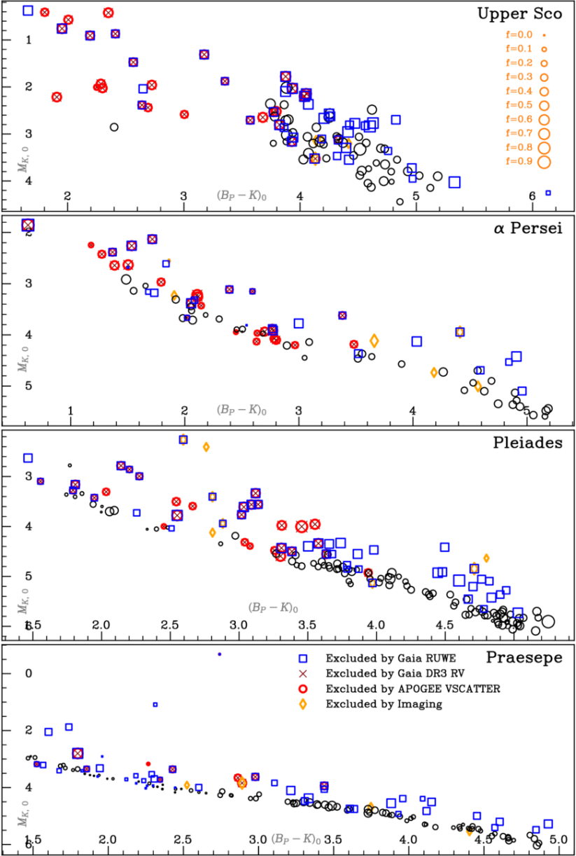
Figure A1. from Lyra Cao and Keivan G. Stassun 2025 Astrophys. J. Lett. 988 doi:10.3847/2041-8213/ade875 https://dx.doi.org/10.3847/2041-8213/ade875 © 2025. The Author(s). Published by the American Astronomical Society.
