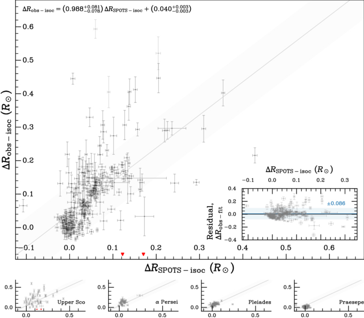
Figure 4. from Lyra Cao and Keivan G. Stassun 2025 Astrophys. J. Lett. 988 doi:10.3847/2041-8213/ade875 https://dx.doi.org/10.3847/2041-8213/ade875 © 2025. The Author(s). Published by the American Astronomical Society.
