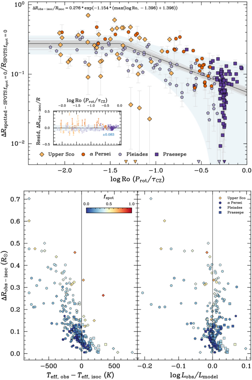
Figure 2. from Lyra Cao and Keivan G. Stassun 2025 Astrophys. J. Lett. 988 doi:10.3847/2041-8213/ade875 https://dx.doi.org/10.3847/2041-8213/ade875 © 2025. The Author(s). Published by the American Astronomical Society.
