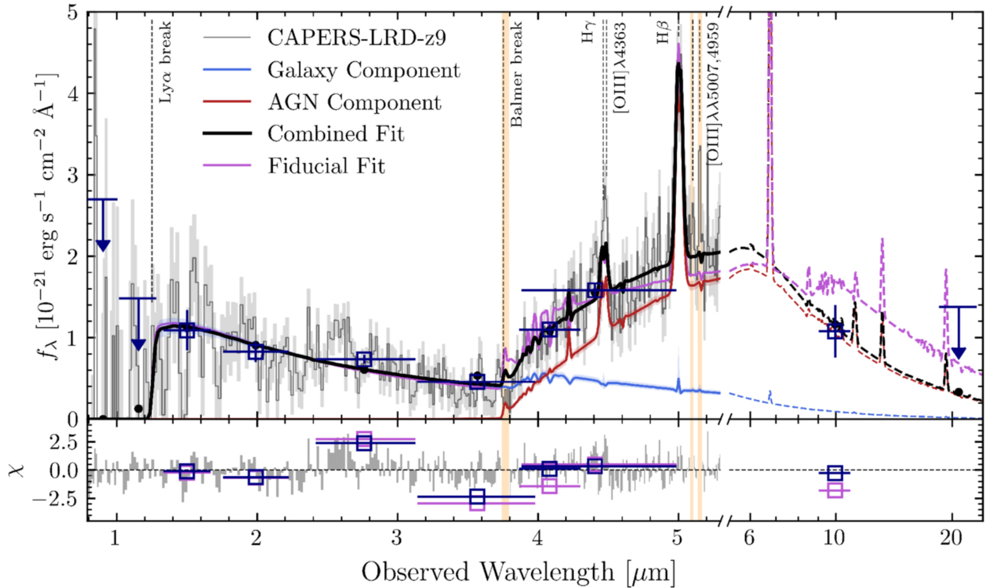
Figure 8. from Anthony J. Taylor et al 2025 Astrophys. J. Lett. 989 doi:10.3847/2041-8213/ade789 https://dx.doi.org/10.3847/2041-8213/ade789 © 2025. The Author(s). Published by the American Astronomical Society.
