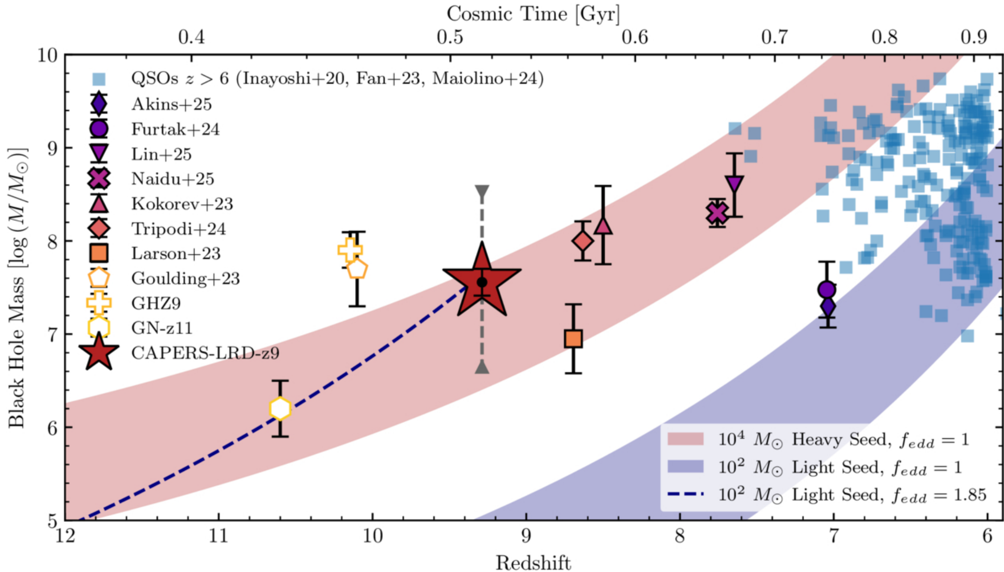
Figure 6. from Anthony J. Taylor et al 2025 Astrophys. J. Lett. 989 doi:10.3847/2041-8213/ade789 https://dx.doi.org/10.3847/2041-8213/ade789 © 2025. The Author(s). Published by the American Astronomical Society.
