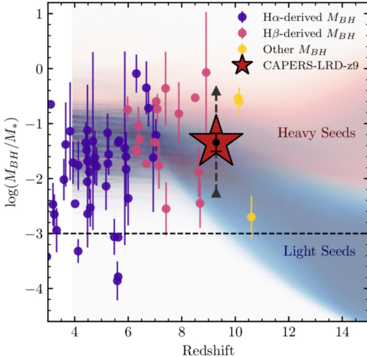
Figure 5. from Anthony J. Taylor et al 2025 Astrophys. J. Lett. 989 doi:10.3847/2041-8213/ade789 https://dx.doi.org/10.3847/2041-8213/ade789 © 2025. The Author(s). Published by the American Astronomical Society.
