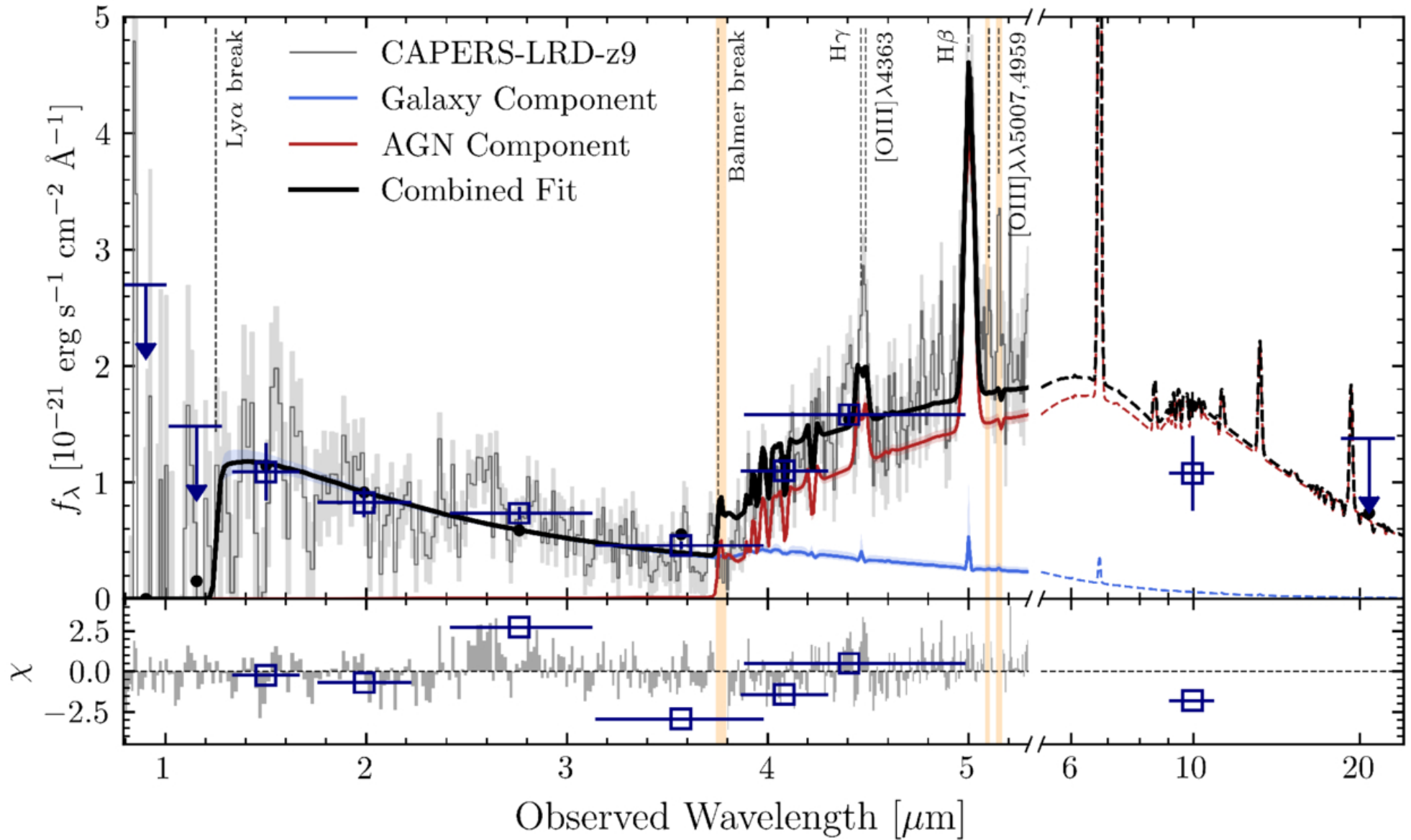
Figure 4. from Anthony J. Taylor et al 2025 Astrophys. J. Lett. 989 doi:10.3847/2041-8213/ade789 https://dx.doi.org/10.3847/2041-8213/ade789 © 2025. The Author(s). Published by the American Astronomical Society.
