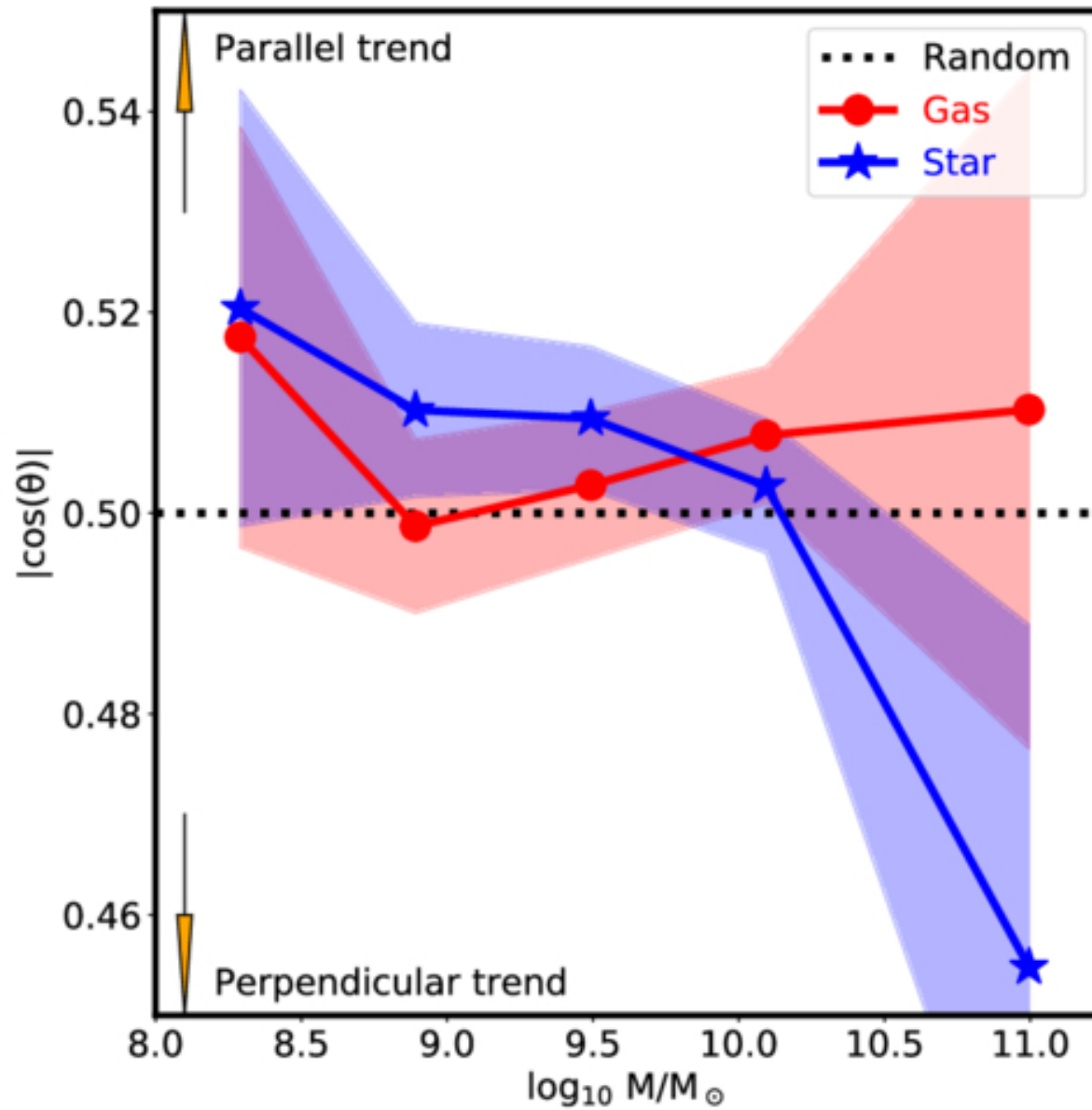
Figure 2. from Hao-da Wang et al 2025 Astrophys. J. Lett. 987 doi:10.3847/2041-8213/ade6fe https://dx.doi.org/10.3847/2041-8213/ade6fe © 2025. The Author(s). Published by the American Astronomical Society.
