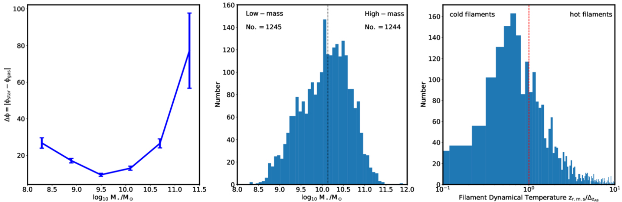
Figure 1. from Hao-da Wang et al 2025 Astrophys. J. Lett. 987 doi:10.3847/2041-8213/ade6fe https://dx.doi.org/10.3847/2041-8213/ade6fe © 2025. The Author(s). Published by the American Astronomical Society.
