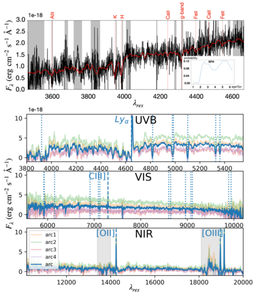
Figure 2. from Rui Li et al 2025 Astrophys. J. Lett. 987 doi:10.3847/2041-8213/ade680 https://dx.doi.org/10.3847/2041-8213/ade680 © 2025. The Author(s). Published by the American Astronomical Society.
