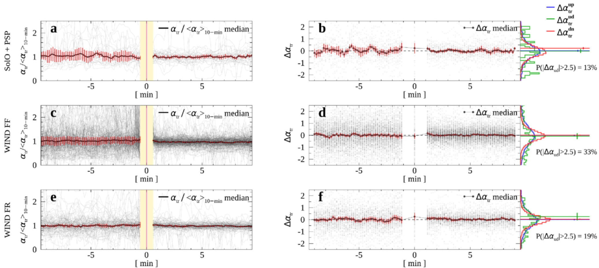
Figure 3. from Byeongseon Park et al 2025 Astrophys. J. Lett. 986 doi:10.3847/2041-8213/ade25b https://dx.doi.org/10.3847/2041-8213/ade25b © 2025. The Author(s). Published by the American Astronomical Society.
