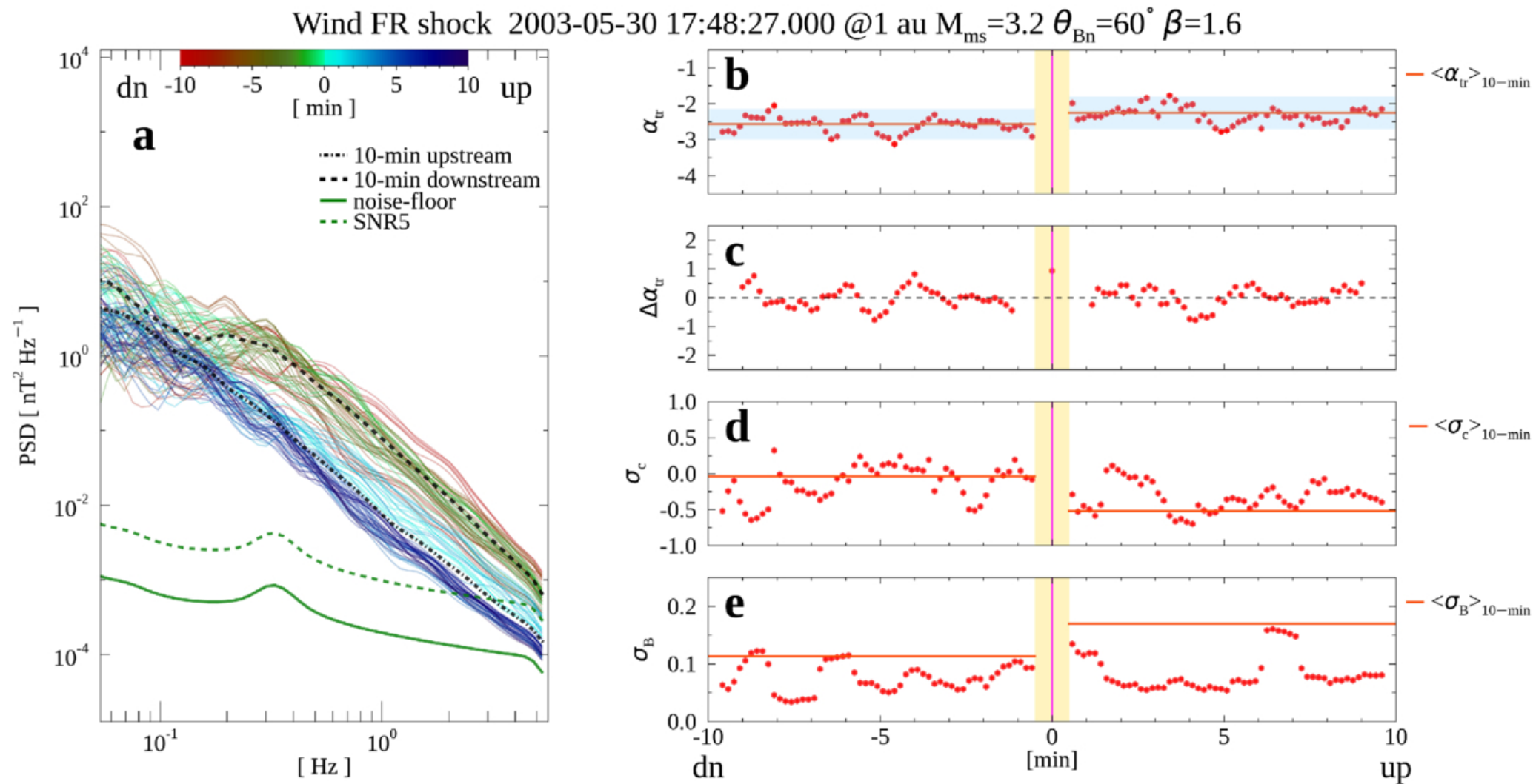
Figure 2. from Byeongseon Park et al 2025 Astrophys. J. Lett. 986 doi:10.3847/2041-8213/ade25b https://dx.doi.org/10.3847/2041-8213/ade25b © 2025. The Author(s). Published by the American Astronomical Society.
