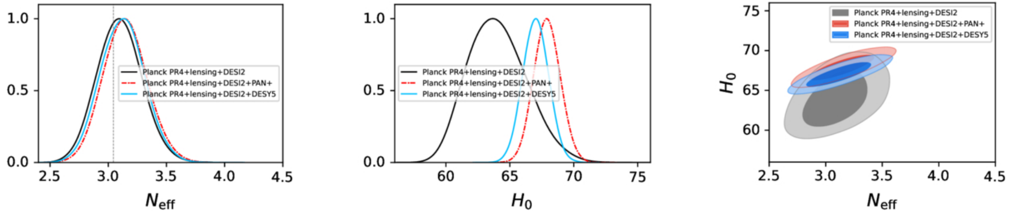
Figure 6. from Shouvik Roy Choudhury 2025 Astrophys. J. Lett. 986 doi:10.3847/2041-8213/ade1cc https://dx.doi.org/10.3847/2041-8213/ade1cc © 2025. The Author(s). Published by the American Astronomical Society.
