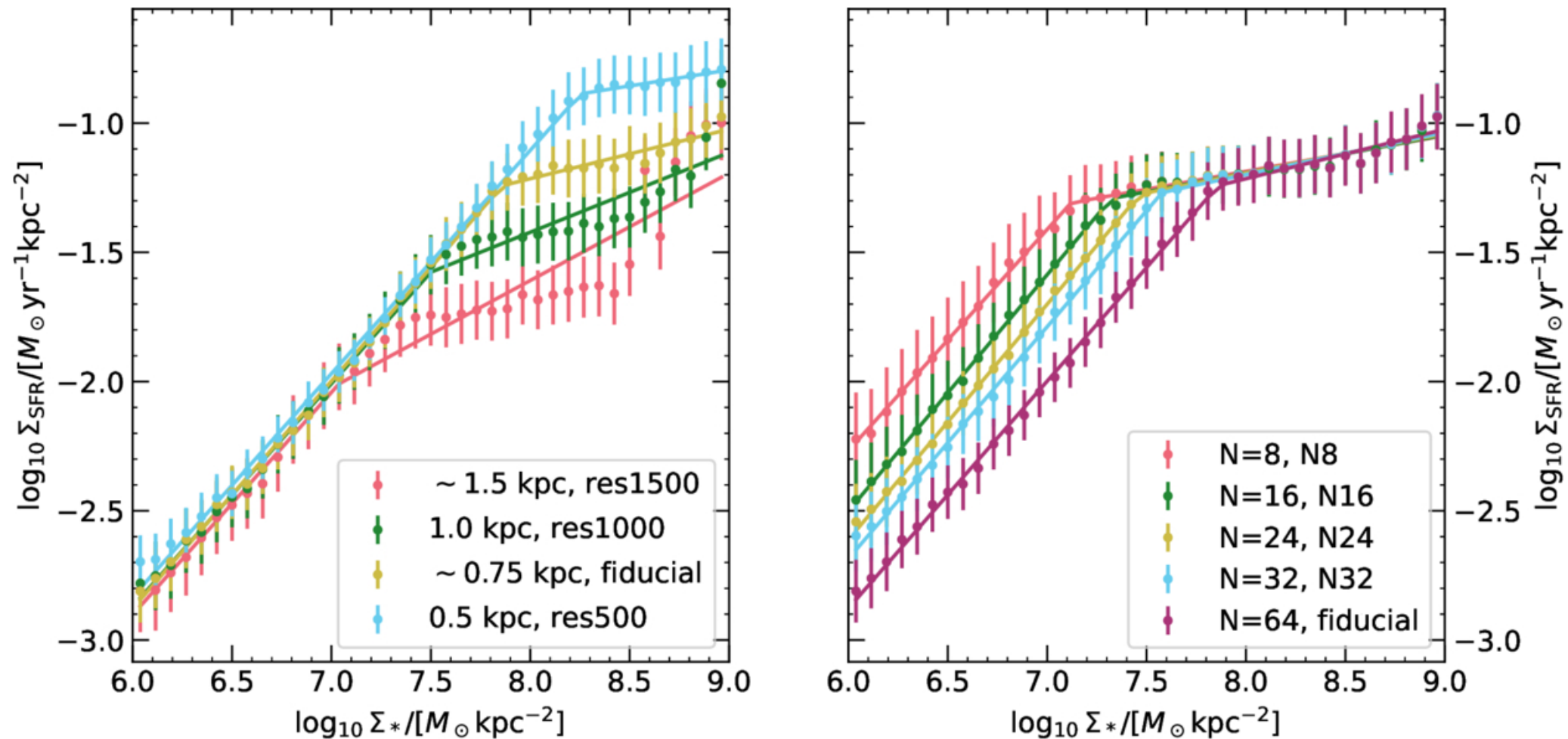
Figure 2. from Bryanne McDonough et al 2025 Astrophys. J. Lett. 986 doi:10.3847/2041-8213/ade13c https://dx.doi.org/10.3847/2041-8213/ade13c © 2025. The Author(s). Published by the American Astronomical Society.
