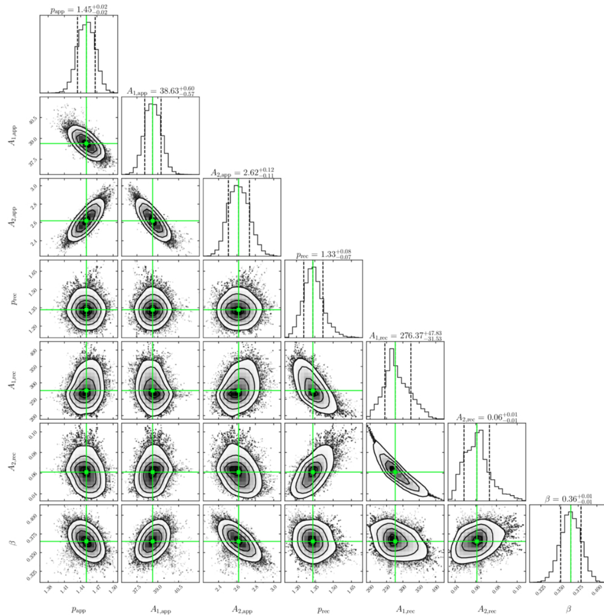
Figure 8. from Andrzej A. Zdziarski et al 2025 Astrophys. J. Lett. 986 doi:10.3847/2041-8213/ade13b https://dx.doi.org/10.3847/2041-8213/ade13b © 2025. The Author(s). Published by the American Astronomical Society.
