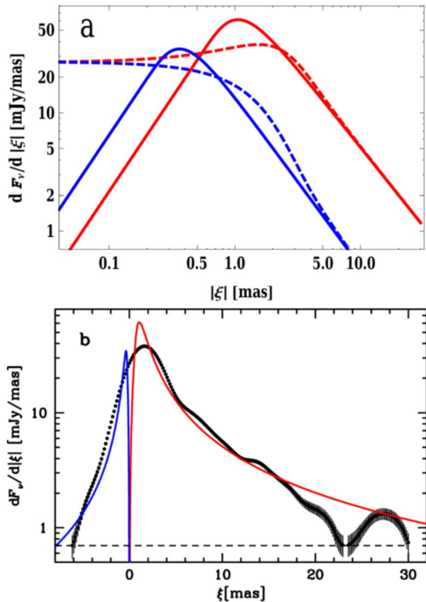
Figure 7. from Andrzej A. Zdziarski et al 2025 Astrophys. J. Lett. 986 doi:10.3847/2041-8213/ade13b https://dx.doi.org/10.3847/2041-8213/ade13b © 2025. The Author(s). Published by the American Astronomical Society.
