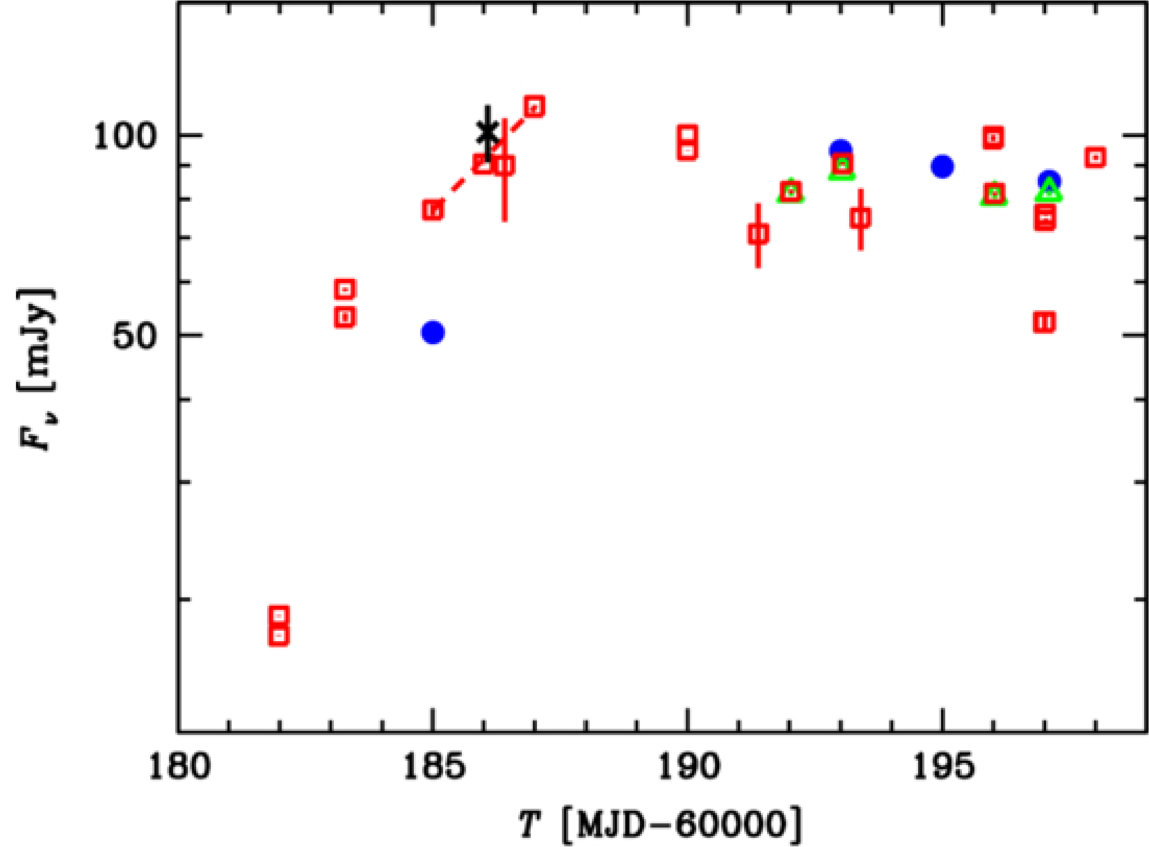
Figure 5. from Andrzej A. Zdziarski et al 2025 Astrophys. J. Lett. 986 doi:10.3847/2041-8213/ade13b https://dx.doi.org/10.3847/2041-8213/ade13b © 2025. The Author(s). Published by the American Astronomical Society.
