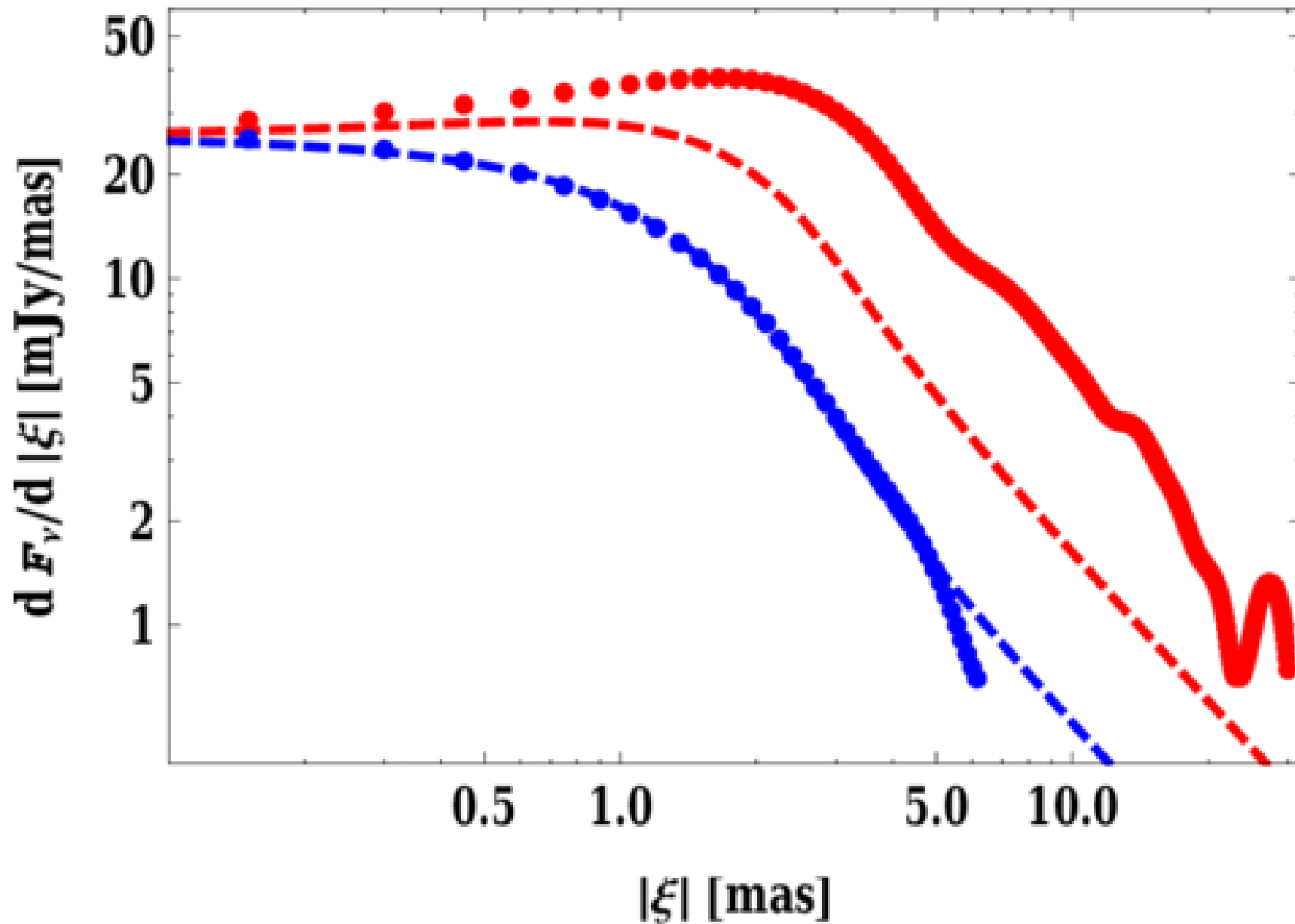
Figure 4. from Andrzej A. Zdziarski et al 2025 Astrophys. J. Lett. 986 doi:10.3847/2041-8213/ade13b https://dx.doi.org/10.3847/2041-8213/ade13b © 2025. The Author(s). Published by the American Astronomical Society.
