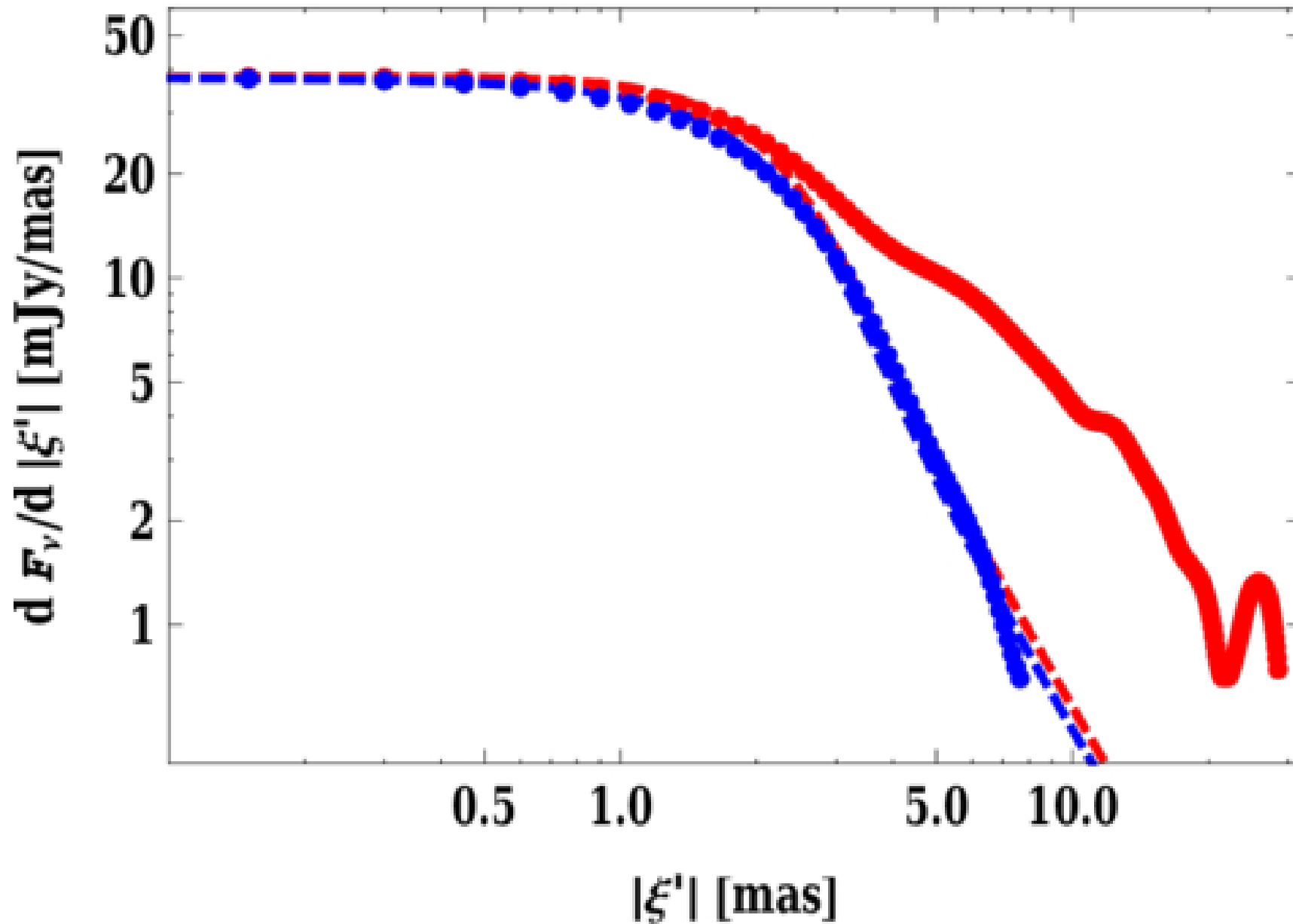
Figure 3. from Andrzej A. Zdziarski et al 2025 Astrophys. J. Lett. 986 doi:10.3847/2041-8213/ade13b https://dx.doi.org/10.3847/2041-8213/ade13b © 2025. The Author(s). Published by the American Astronomical Society.
