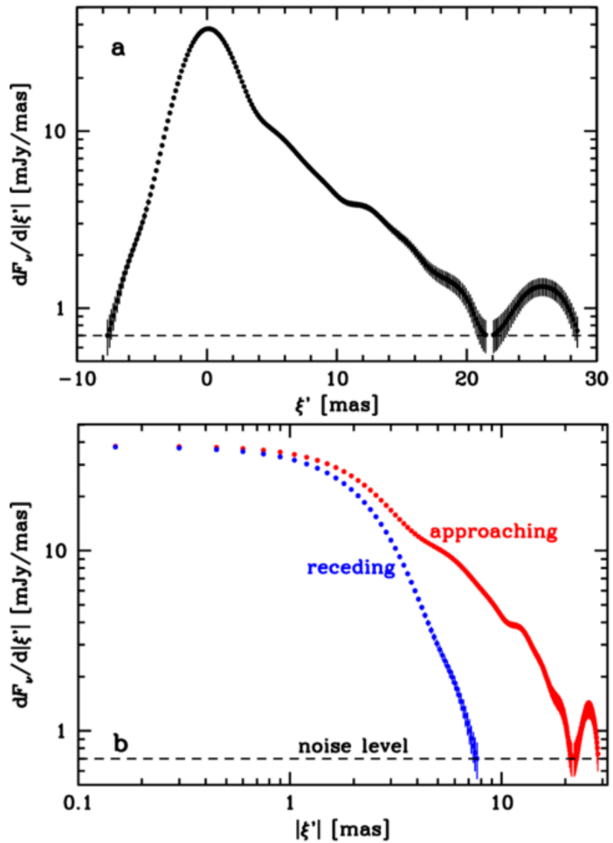
Figure 2. from Andrzej A. Zdziarski et al 2025 Astrophys. J. Lett. 986 doi:10.3847/2041-8213/ade13b https://dx.doi.org/10.3847/2041-8213/ade13b © 2025. The Author(s). Published by the American Astronomical Society.
