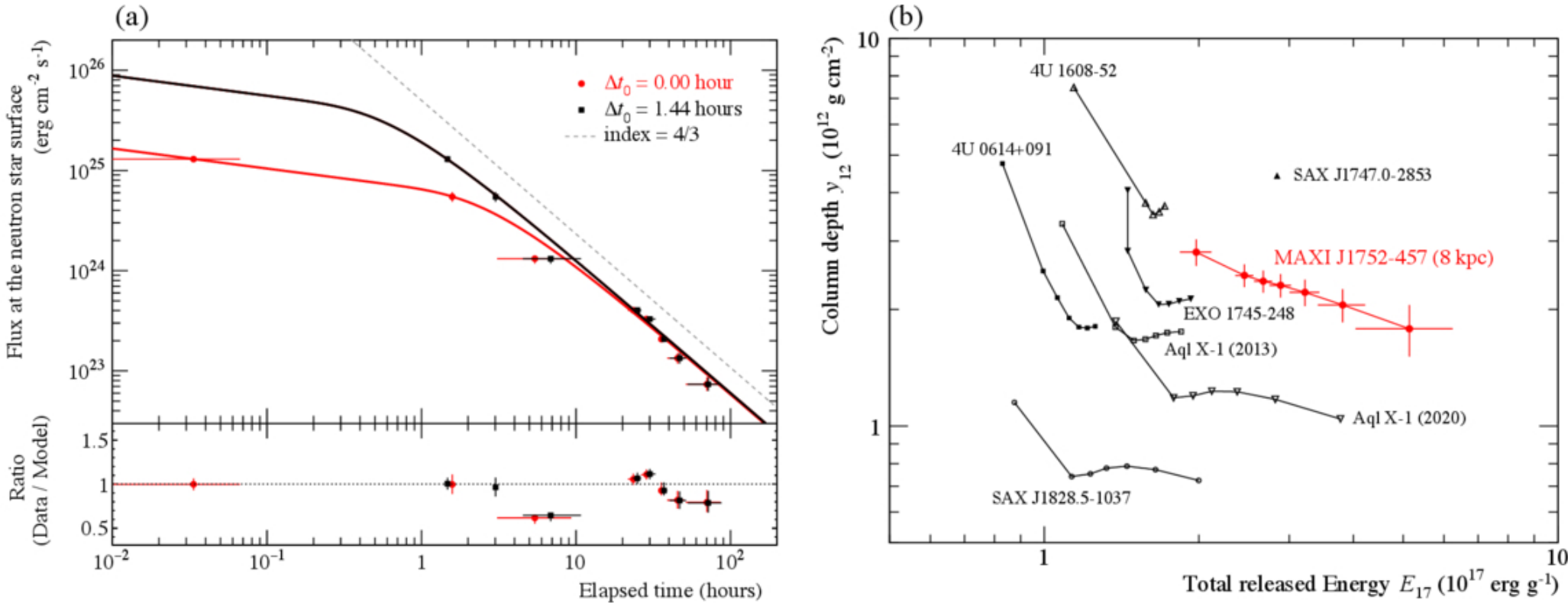
Figure 4. from Amira Aoyama et al 2025 Astrophys. J. Lett. 986 doi:10.3847/2041-8213/addd00 https://dx.doi.org/10.3847/2041-8213/addd00 © 2025. The Author(s). Published by the American Astronomical Society.
