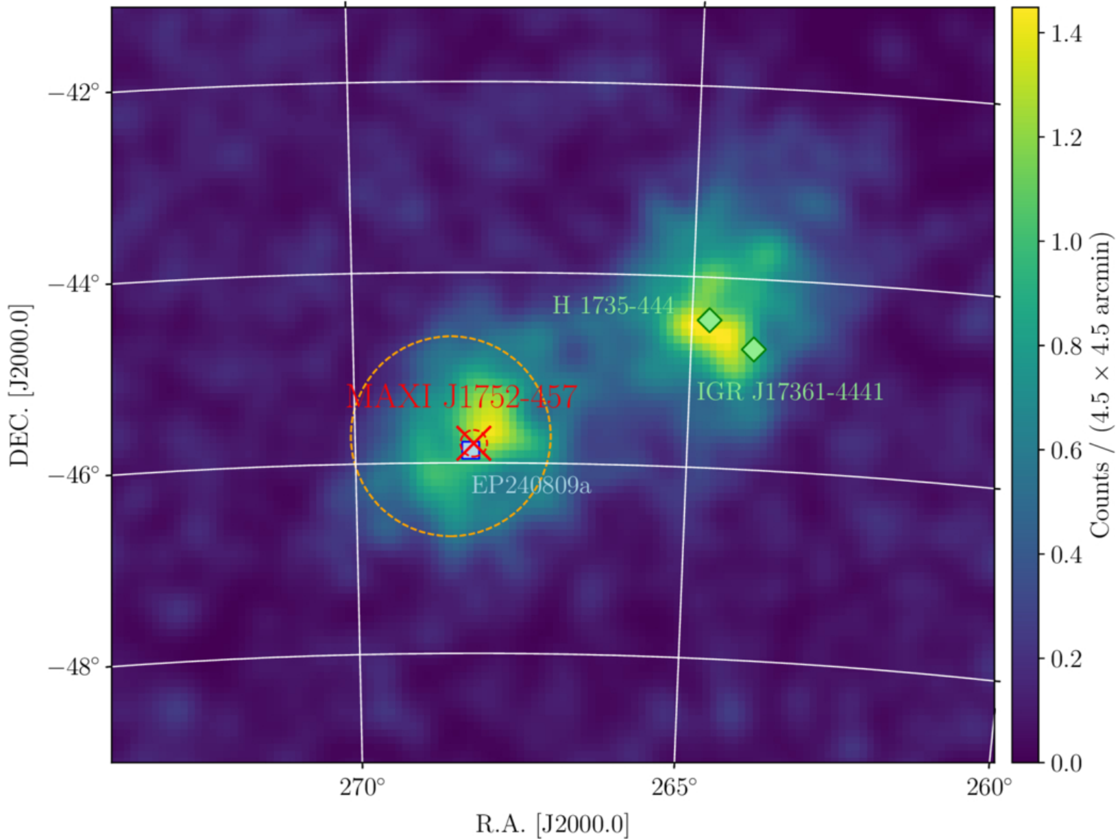
Figure 1. from Amira Aoyama et al 2025 Astrophys. J. Lett. 986 doi:10.3847/2041-8213/addd00 https://dx.doi.org/10.3847/2041-8213/addd00 © 2025. The Author(s). Published by the American Astronomical Society.
