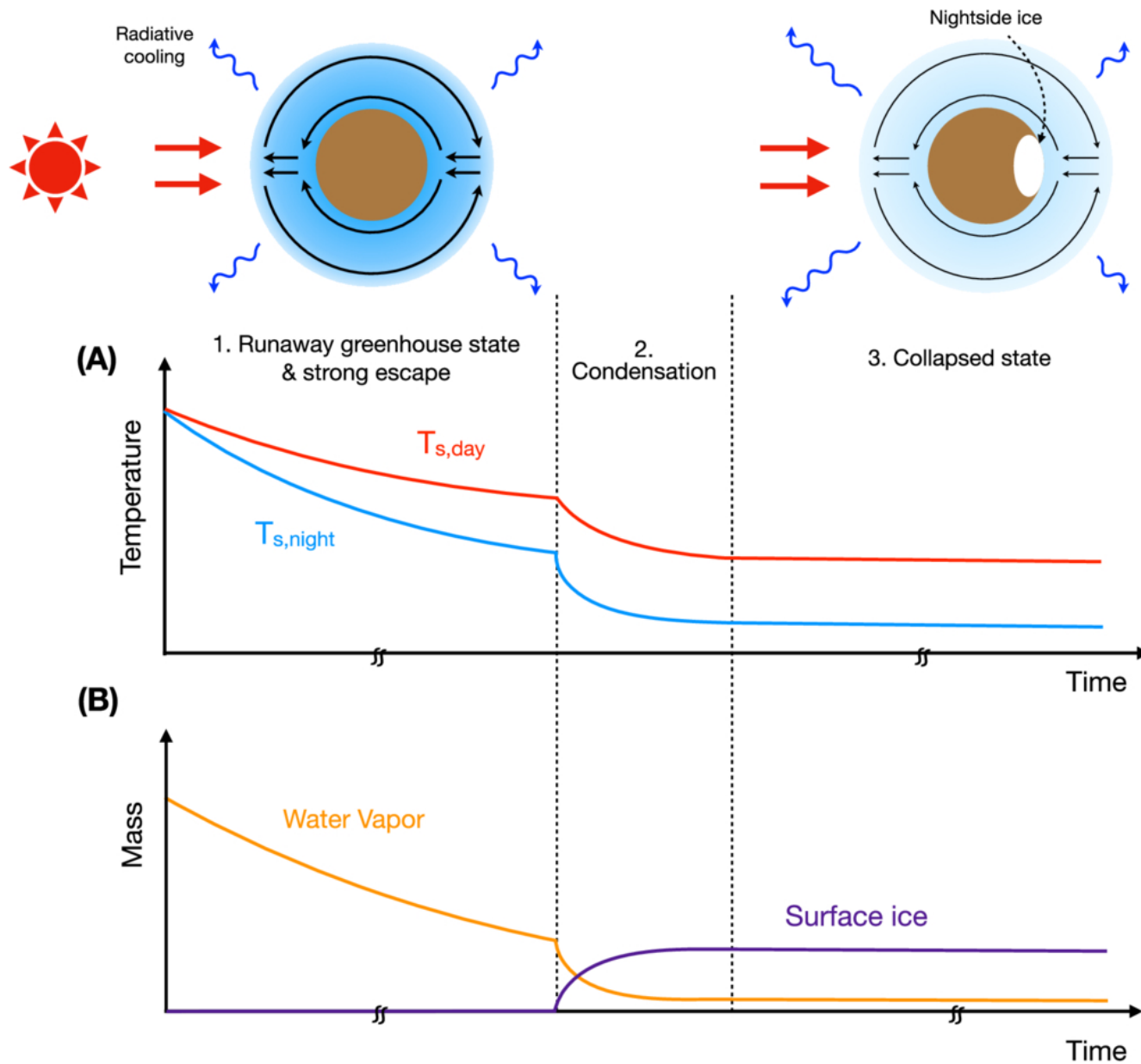
Figure 1. from Yueyun Ouyang et al 2025 Astrophys. J. Lett. 985 doi:10.3847/2041-8213/adda4b https://dx.doi.org/10.3847/2041-8213/adda4b © 2025. The Author(s). Published by the American Astronomical Society.
