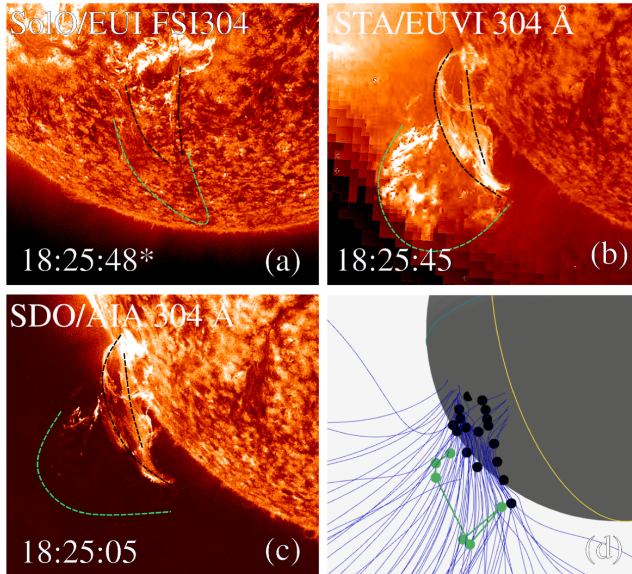
Figure 6. from Abril Sahade et al 2025 Astrophys. J. Lett. 986 doi:10.3847/2041-8213/add939 https://dx.doi.org/10.3847/2041-8213/add939 © 2025. The Author(s). Published by the American Astronomical Society.
