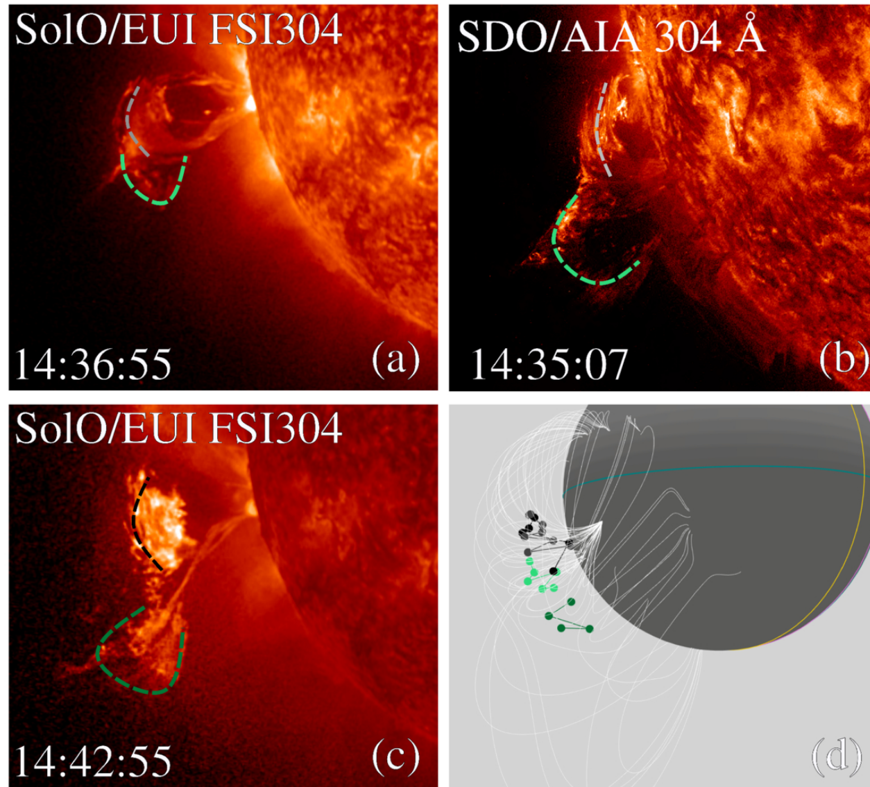
Figure 4. from Abril Sahade et al 2025 Astrophys. J. Lett. 986 doi:10.3847/2041-8213/add939 https://dx.doi.org/10.3847/2041-8213/add939 © 2025. The Author(s). Published by the American Astronomical Society.
