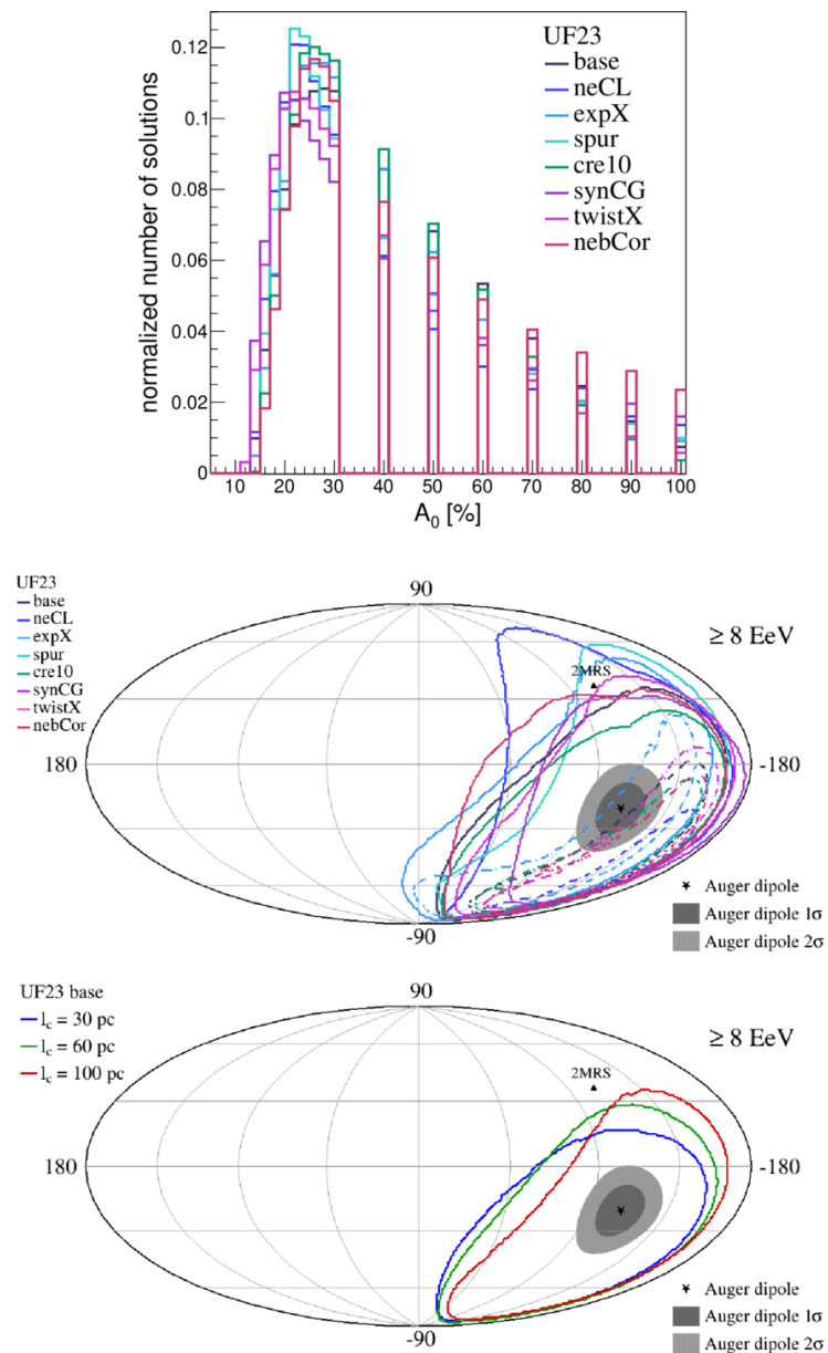
Figure 9. from Jakub Vicha et al 2025 Astrophys. J. Lett. 986 doi:10.3847/2041-8213/add536 https://dx.doi.org/10.3847/2041-8213/add536 © 2025. The Author(s). Published by the American Astronomical Society.
