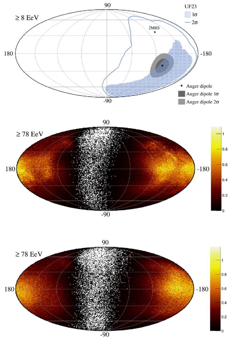
Figure 5. from Jakub Vicha et al 2025 Astrophys. J. Lett. 986 doi:10.3847/2041-8213/add536 https://dx.doi.org/10.3847/2041-8213/add536 © 2025. The Author(s). Published by the American Astronomical Society.
