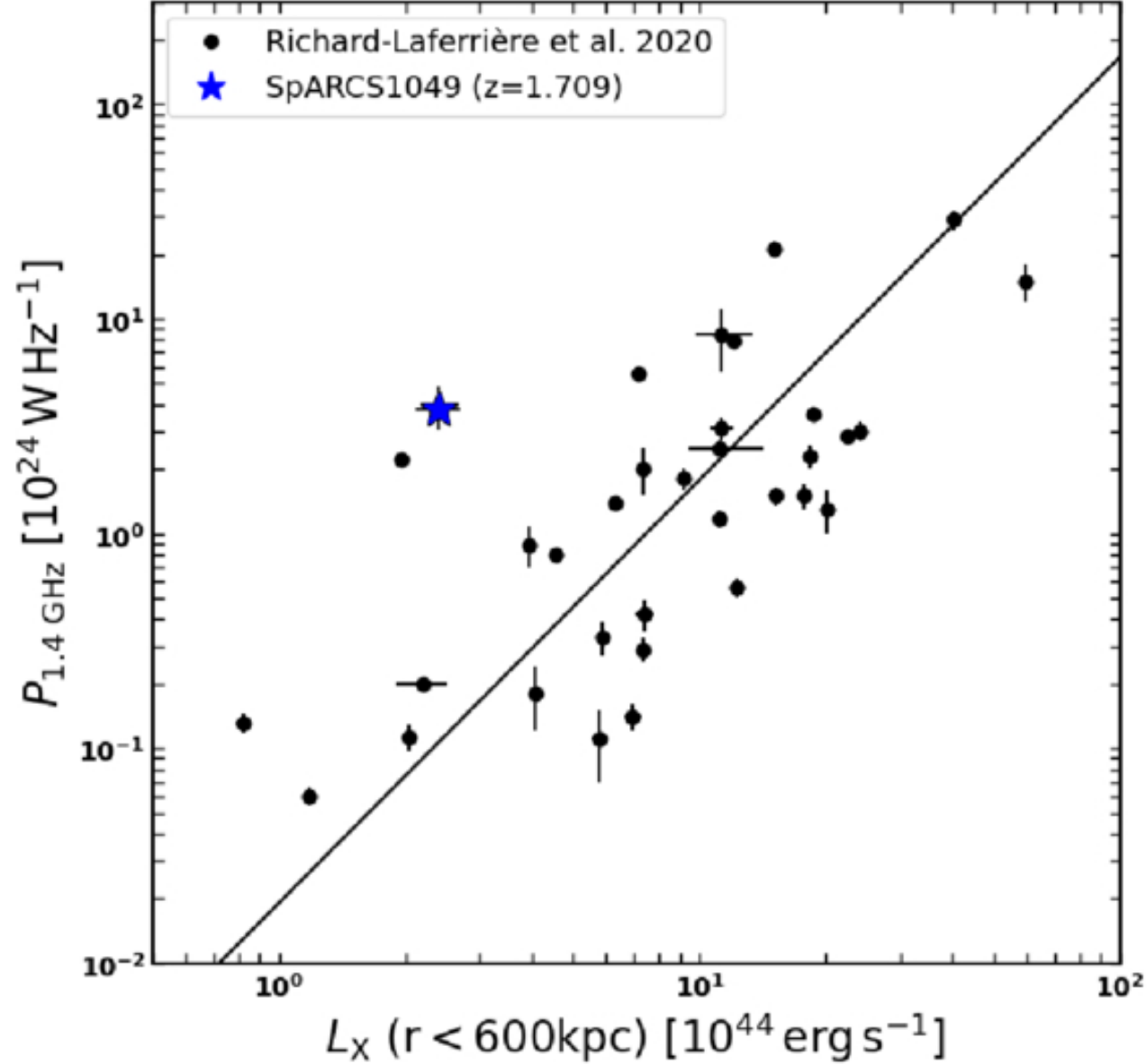
Figure 4. from Julie HLavacek-Larrondo et al 2025 Astrophys. J. Lett. 987 doi:10.3847/2041-8213/add527 https://dx.doi.org/10.3847/2041-8213/add527 © 2025. The Author(s). Published by the American Astronomical Society.
