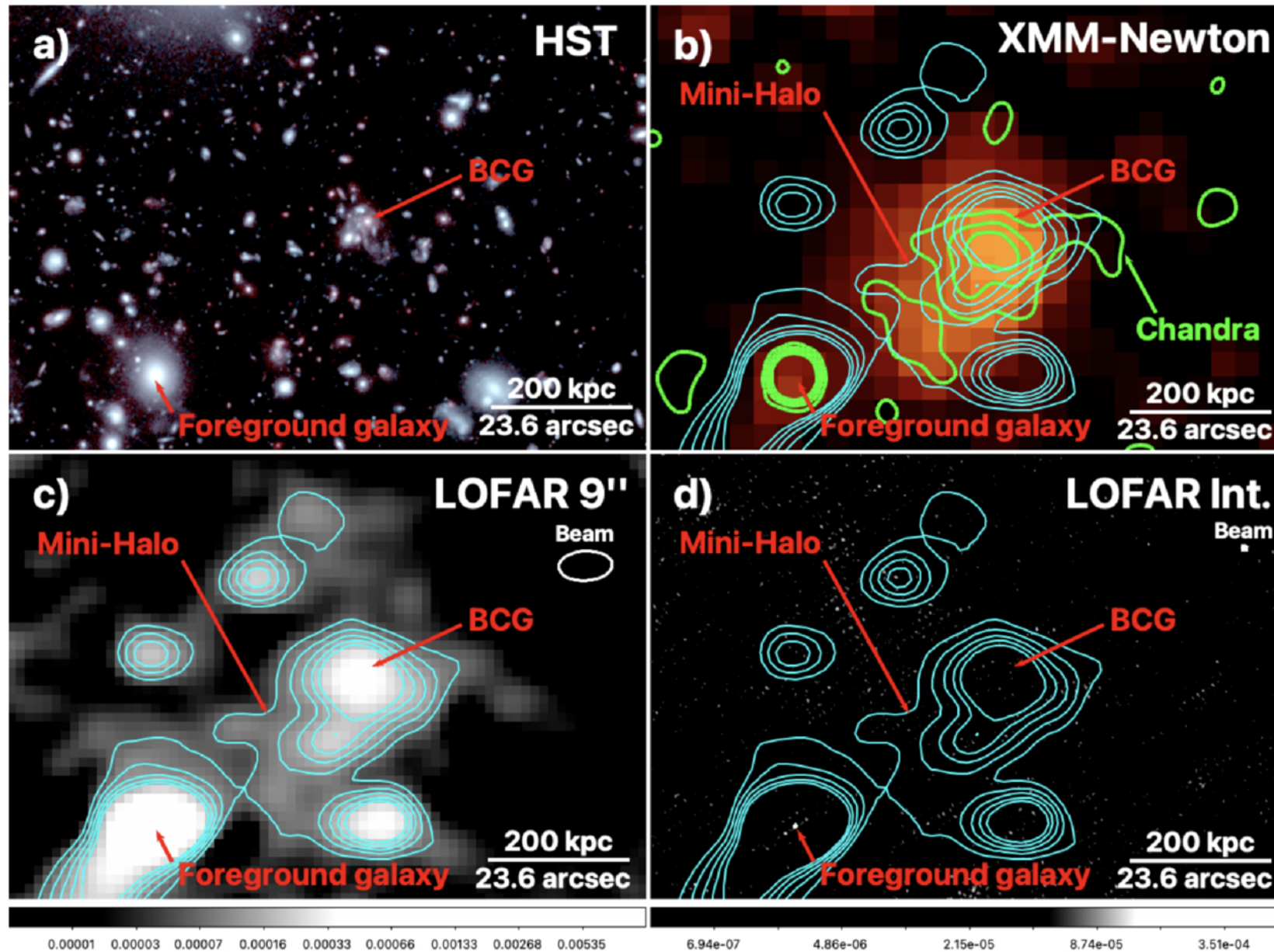
Figure 1. from Julie HLavacek-Larrondo et al 2025 Astrophys. J. Lett. 987 doi:10.3847/2041-8213/add527 https://dx.doi.org/10.3847/2041-8213/add527 © 2025. The Author(s). Published by the American Astronomical Society.
