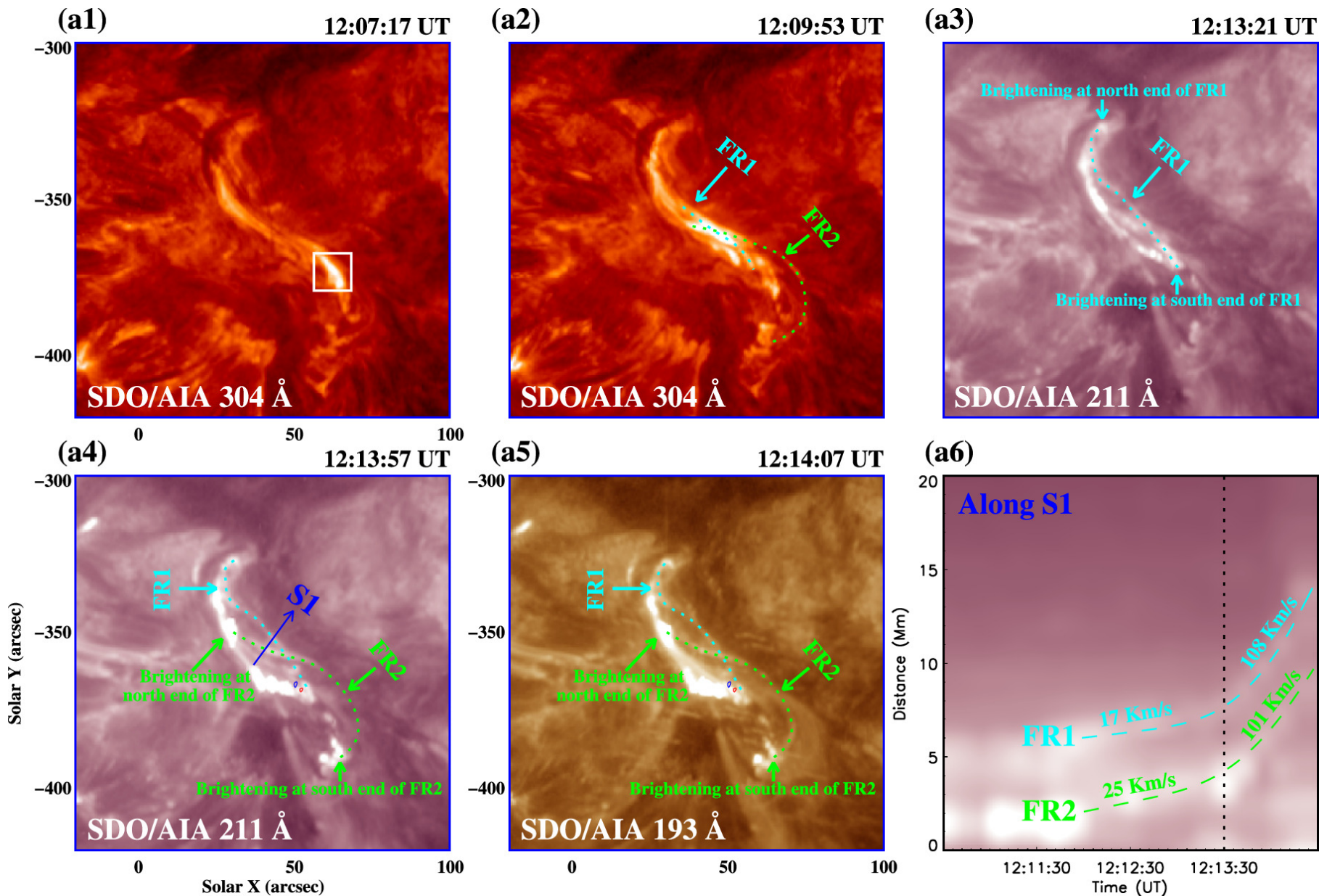
Figure 3. from Tao Ding et al 2025 Astrophys. J. Lett. 985 doi:10.3847/2041-8213/add32c https://dx.doi.org/10.3847/2041-8213/add32c © 2025. The Author(s). Published by the American Astronomical Society.
