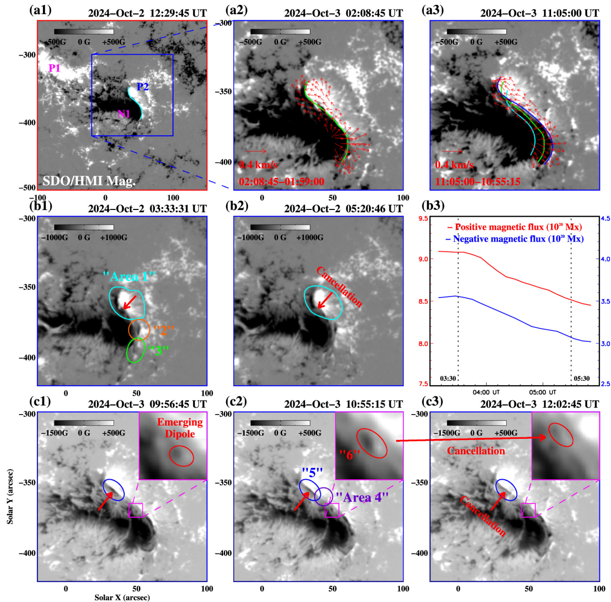
Figure 2. from Tao Ding et al 2025 Astrophys. J. Lett. 985 doi:10.3847/2041-8213/add32c https://dx.doi.org/10.3847/2041-8213/add32c © 2025. The Author(s). Published by the American Astronomical Society.
