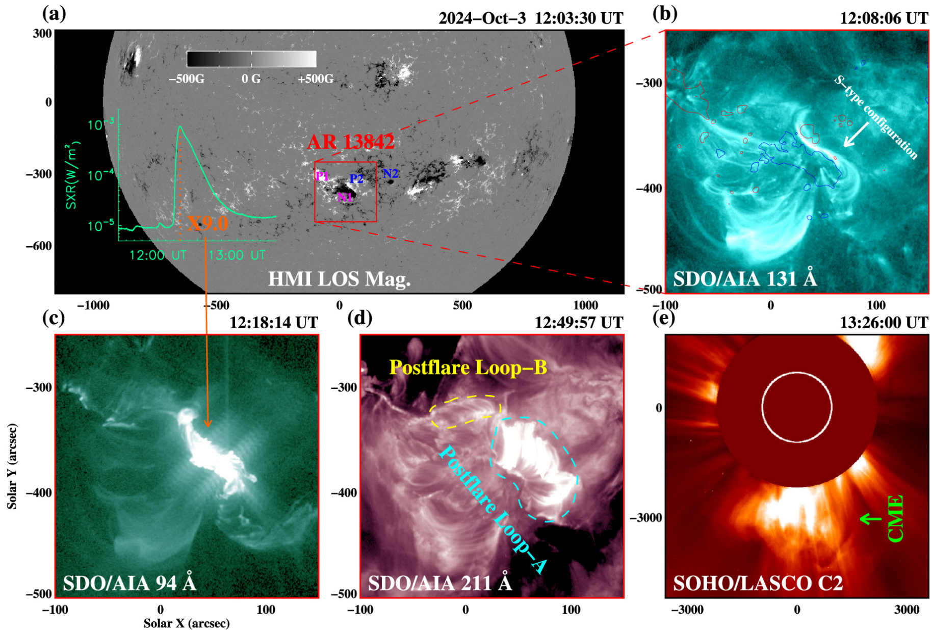
Figure 1. from Tao Ding et al 2025 Astrophys. J. Lett. 985 doi:10.3847/2041-8213/add32c https://dx.doi.org/10.3847/2041-8213/add32c © 2025. The Author(s). Published by the American Astronomical Society.
