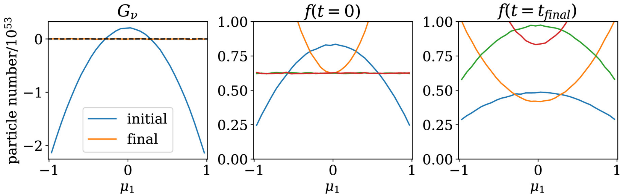
Figure 7. from Kelsey A. Lund et al 2025 Astrophys. J. Lett. 985 doi:10.3847/2041-8213/add0a7 https://dx.doi.org/10.3847/2041-8213/add0a7 © 2025. The Author(s). Published by the American Astronomical Society.
