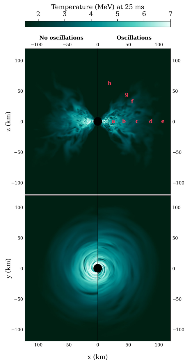
Figure 2. from Kelsey A. Lund et al 2025 Astrophys. J. Lett. 985 doi:10.3847/2041-8213/add0a7 https://dx.doi.org/10.3847/2041-8213/add0a7 © 2025. The Author(s). Published by the American Astronomical Society.
