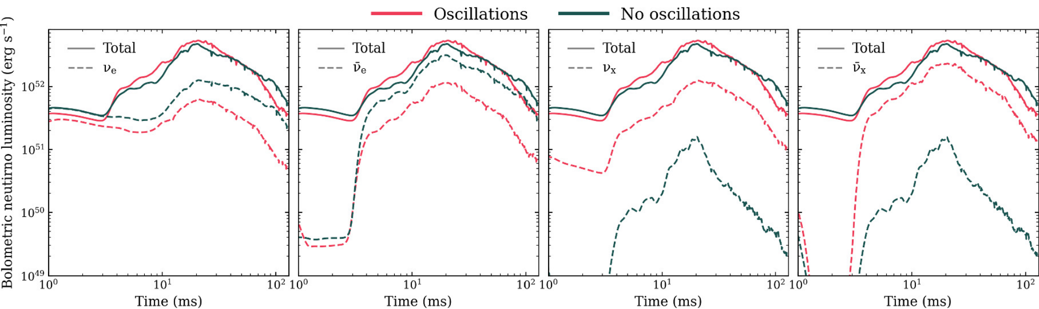
Figure 1. from Kelsey A. Lund et al 2025 Astrophys. J. Lett. 985 doi:10.3847/2041-8213/add0a7 https://dx.doi.org/10.3847/2041-8213/add0a7 © 2025. The Author(s). Published by the American Astronomical Society.
