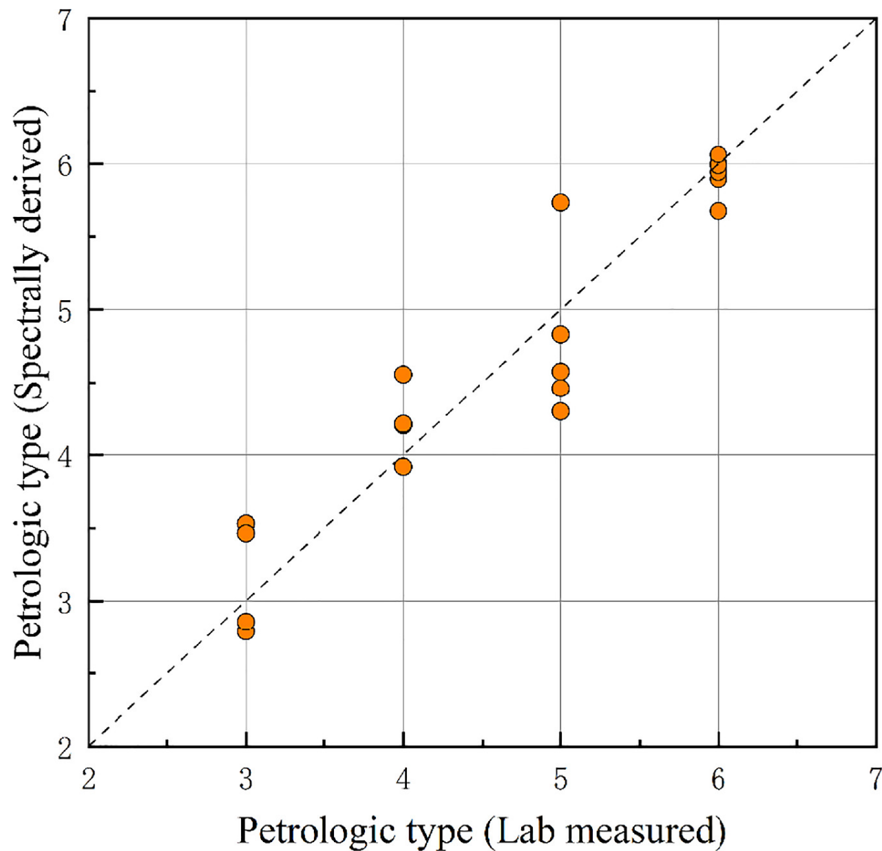
Figure 3. from Pengyue Wang et al 2025 Astrophys. J. Lett. 985 doi:10.3847/2041-8213/adce6e https://dx.doi.org/10.3847/2041-8213/adce6e © 2025. The Author(s). Published by the American Astronomical Society.
