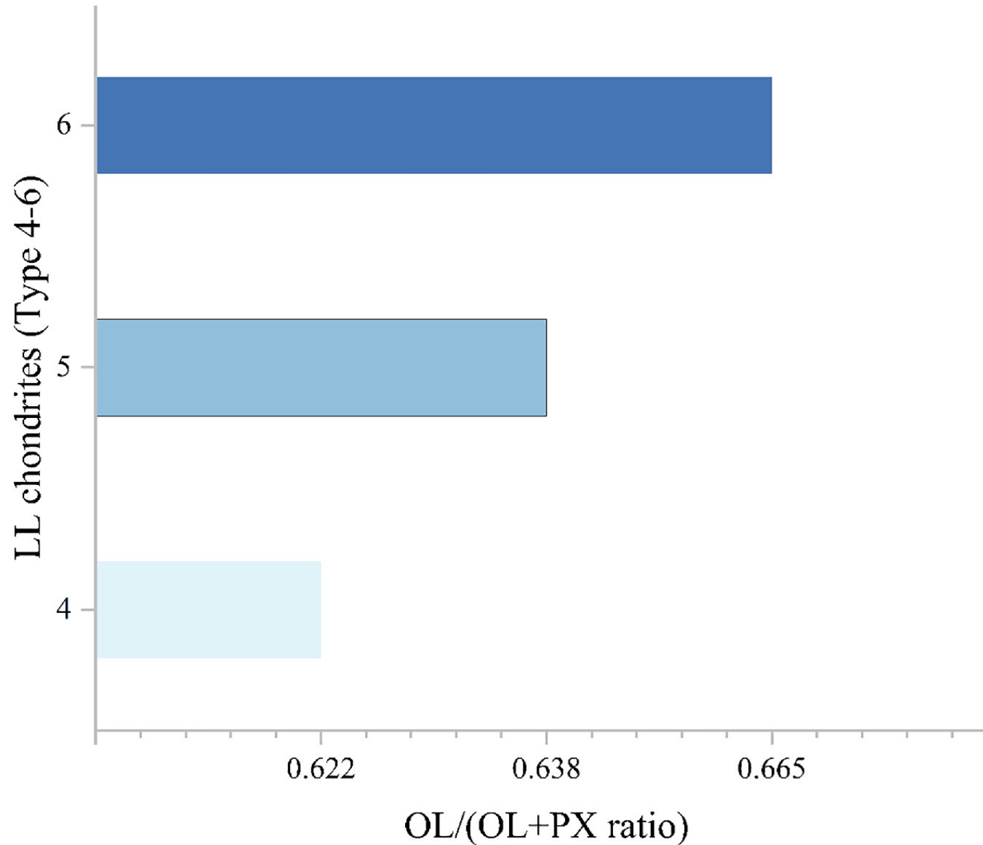
Figure 2. from Pengyue Wang et al 2025 Astrophys. J. Lett. 985 doi:10.3847/2041-8213/adce6e https://dx.doi.org/10.3847/2041-8213/adce6e © 2025. The Author(s). Published by the American Astronomical Society.
