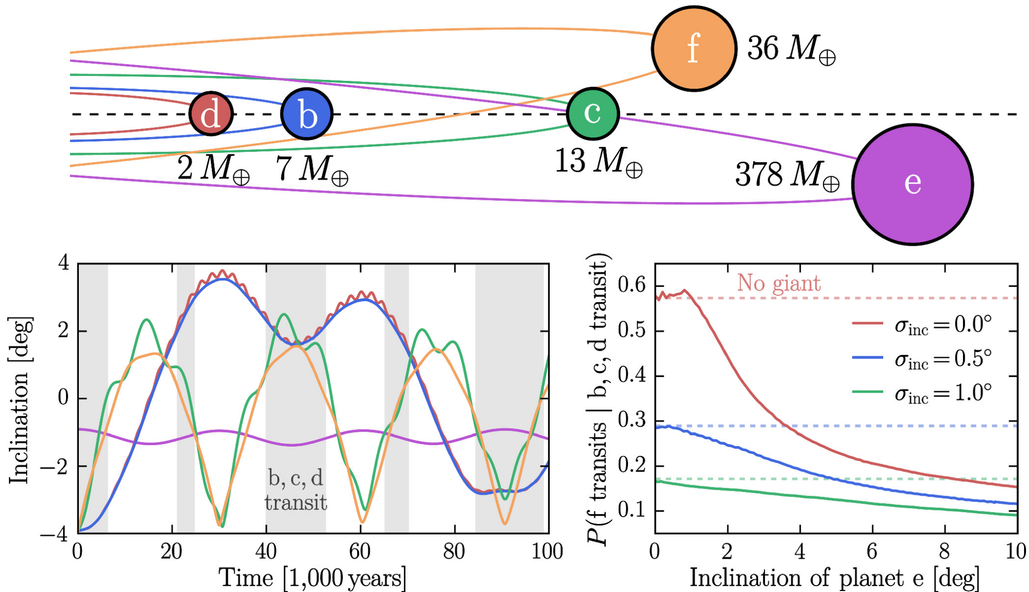
Figure 5. from Caleb Lammers and Joshua N. Winn 2025 Astrophys. J. Lett. 984 doi:10.3847/2041-8213/adce01 https://dx.doi.org/10.3847/2041-8213/adce01 © 2025. The Author(s). Published by the American Astronomical Society.
