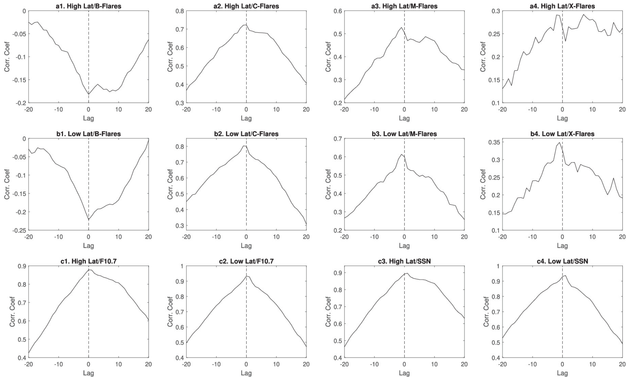
Figure 3. from Jacob Oloketuyi et al 2025 Astrophys. J. Lett. 984 doi:10.3847/2041-8213/adcb38 https://dx.doi.org/10.3847/2041-8213/adcb38 © 2025. The Author(s). Published by the American Astronomical Society.
